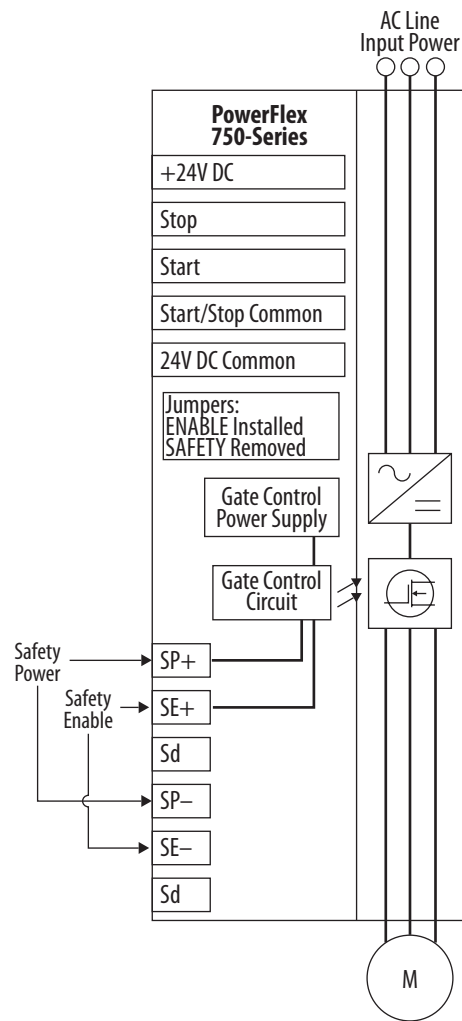
Figure 1 - Drive Safe Torque Off Circuitry
