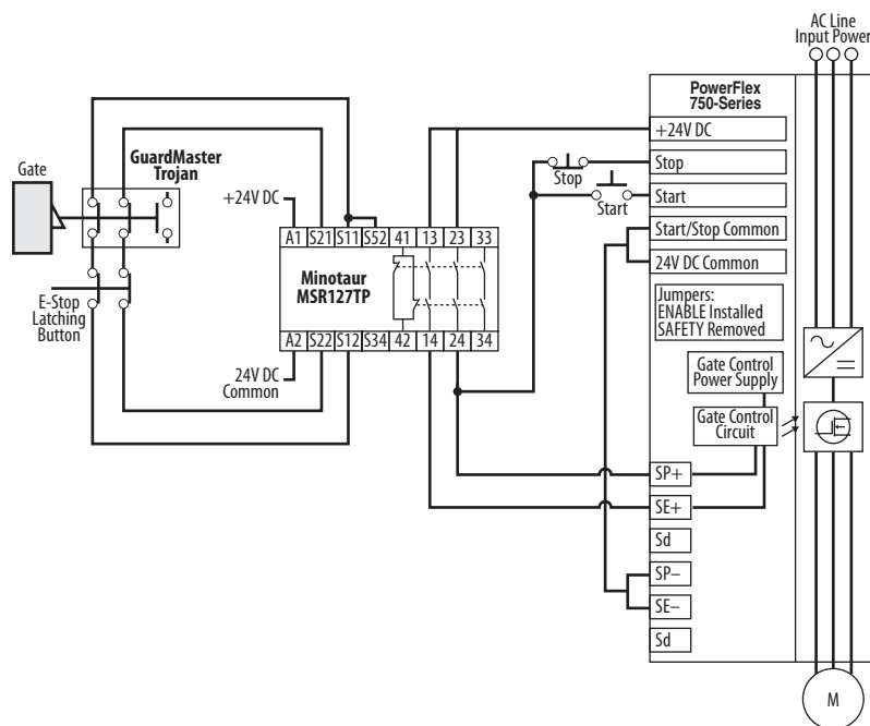
Figure 2 - Stop Category 0 – Coast
