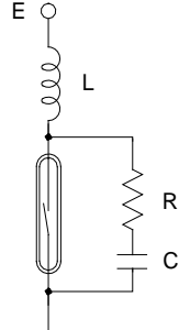
Protecting Circuit Using CR
