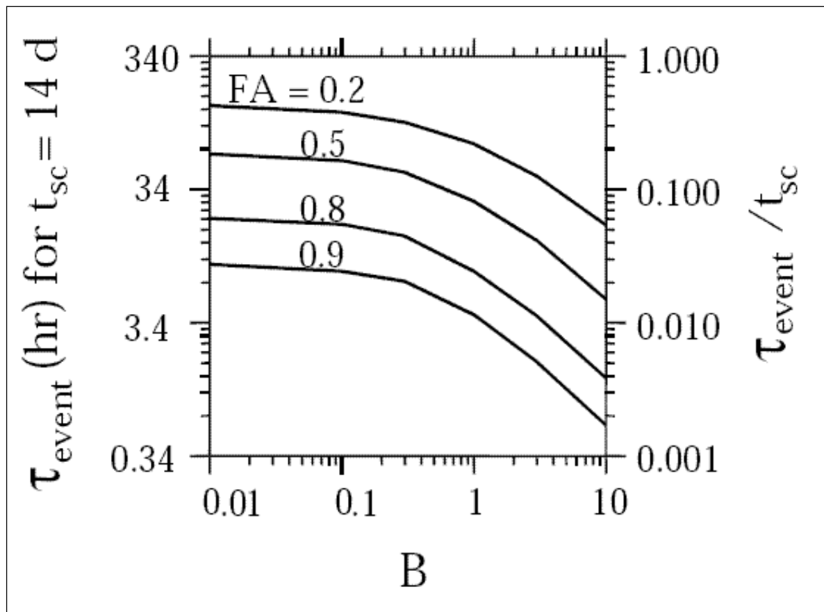
Figure 41: FA as a function of B and \tau_{event} ( t_{sc} equals the average turnover time of the stratum corneum and has a default value of 14 days)
