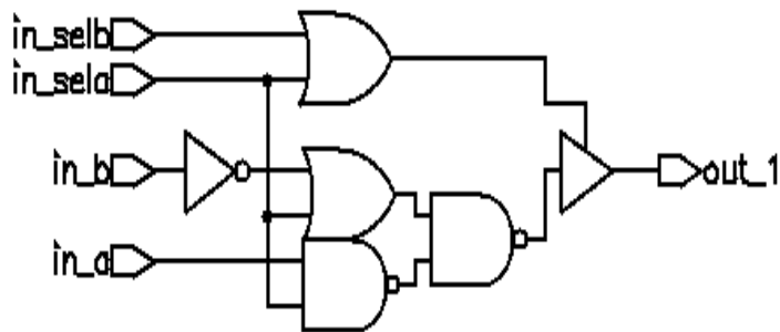
Figure 4-23 Three-State Driver With Gated Data
