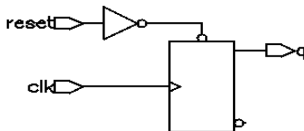
Figure 4-9 Toggle Flip-Flop With Asynchronous Reset
