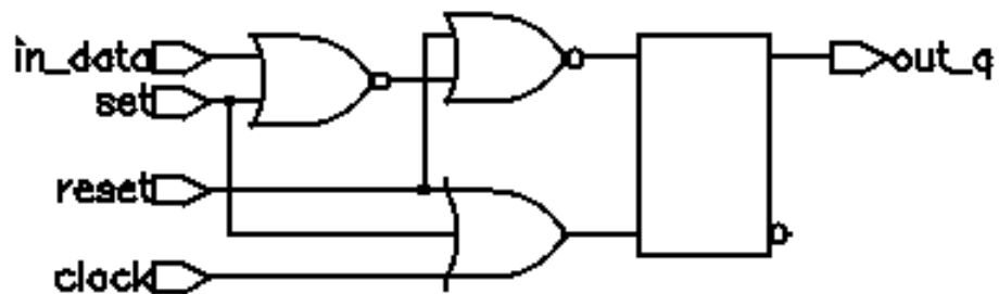
Figure 4-18 Latch With Active-High Set and Reset
