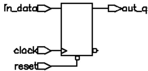
Figure 4-3 D Flip-Flop With an Active-Low Asynchronous Reset
