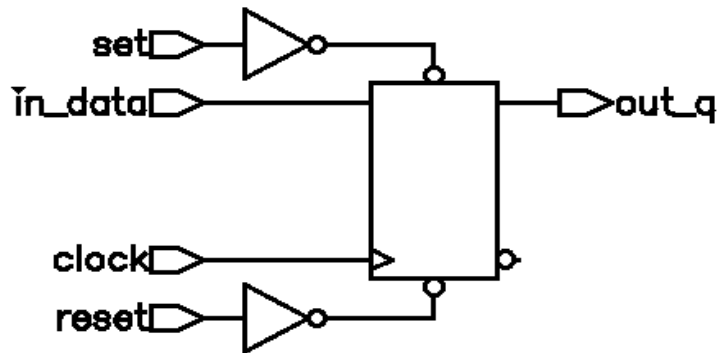
Figure 4-4 Flip-Flop With Asynchronous Set and Reset
