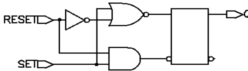
Figure 4-11 SR Latch
