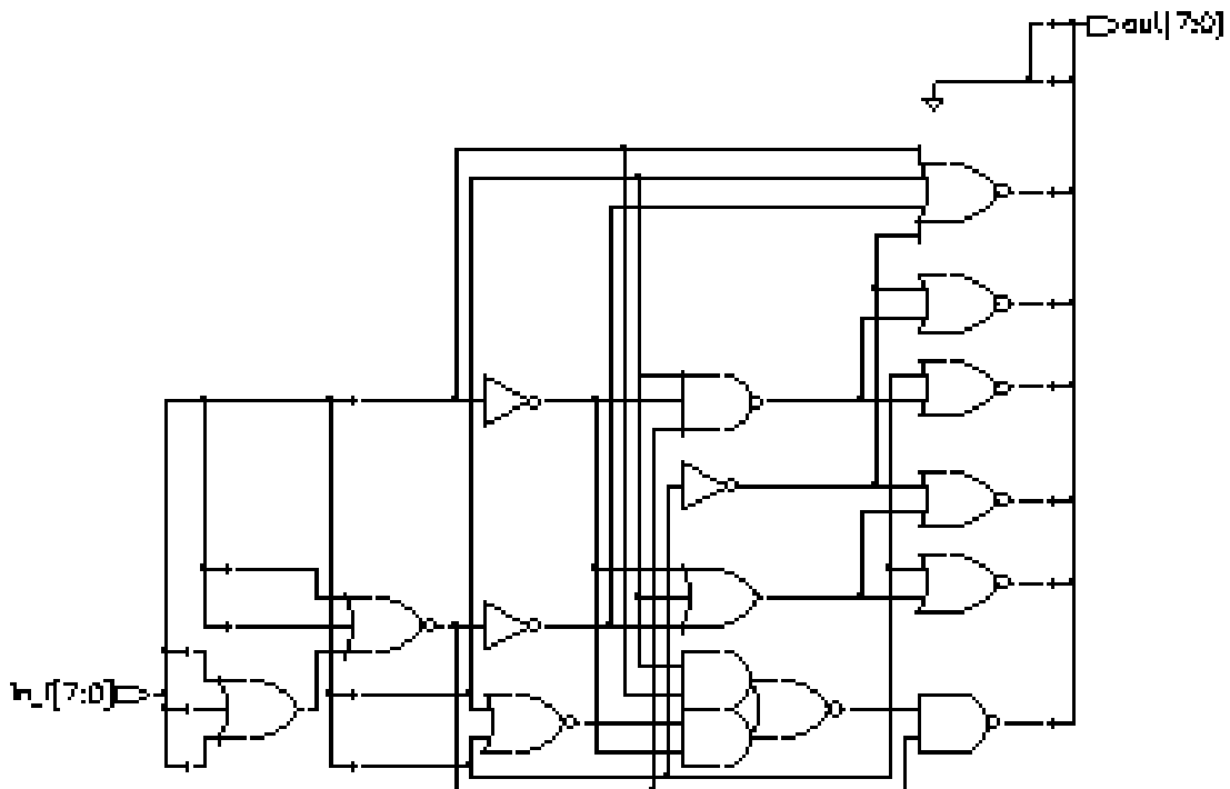
Figure 4-15 Avoiding Latch Inference by Adding a Default Case to a switch Statement
