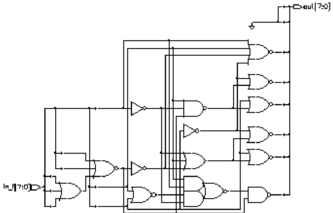
Figure 4-16 Avoiding Latch Inference by Setting a Default Case Before a switch Statement
