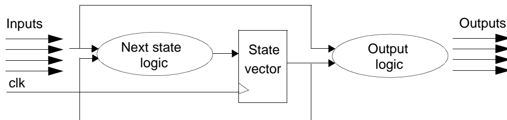
Figure 4-26 Mealy State Machine
