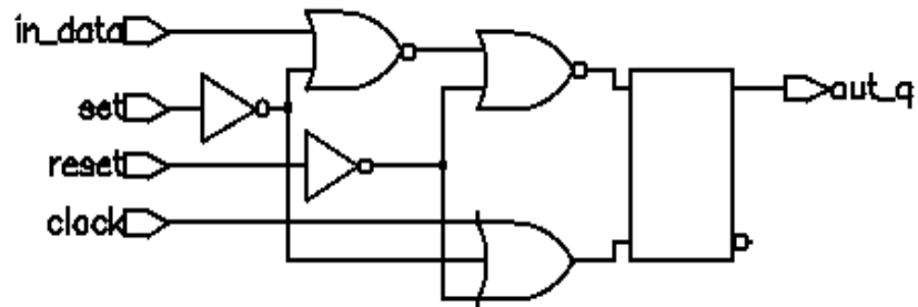
Figure 4-19 Latch With Asynchronous Set and Reset
