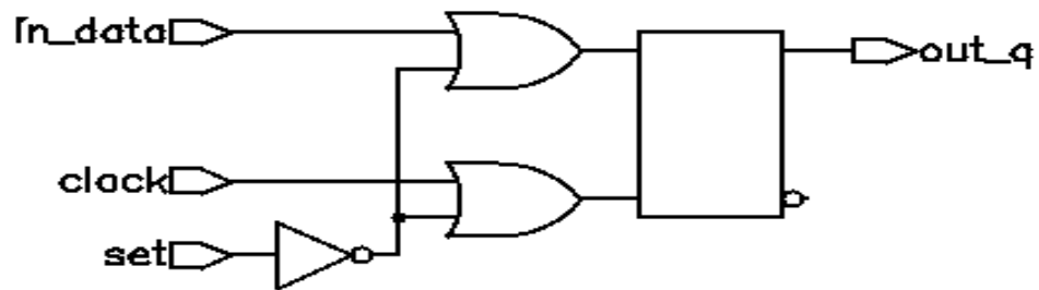
Figure 4-20 Latch With Asynchronous Set
