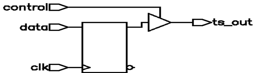
Figure 4-25 Three-State Driver Without Registered Enable
