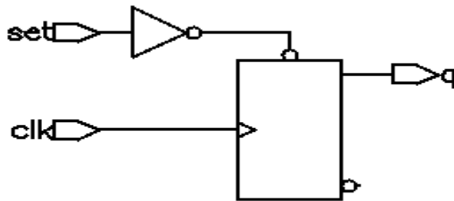
Figure 4-8 Toggle Flip-Flop With Asynchronous Set
