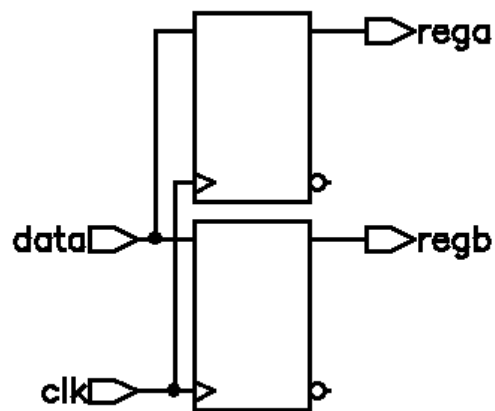
Figure 2-5 Variable Assignment Schematic
