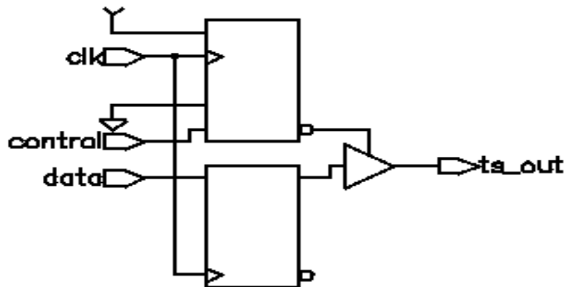
Figure 4-24 Three-State Driver With Registered Enable
