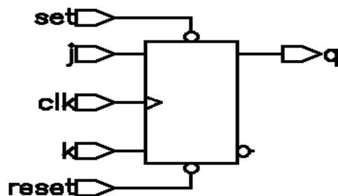
Figure 4-7 JK Flip-Flop With Asynchronous Set and Reset
