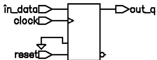
Figure 4-5 D Flip-Flop With Synchronous Reset
