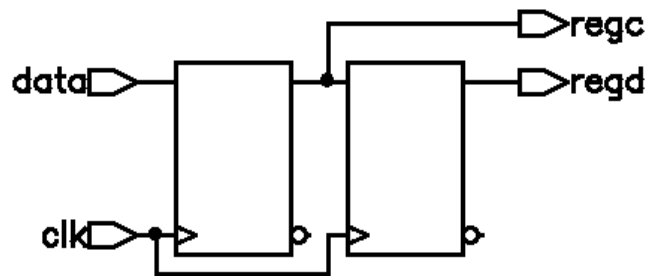
Figure 2-4 Signal Assignment Schematic
