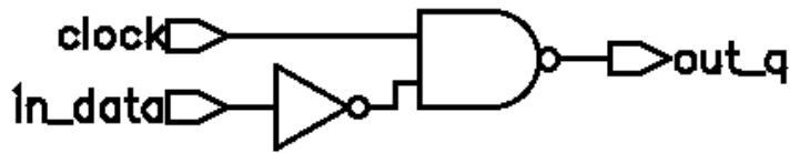
Figure 4-13 Avoiding Latch Inference by a Default Value
