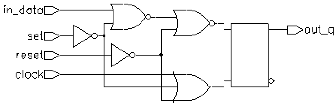
Figure 4-17 Latch With Active-Low Set and Reset
