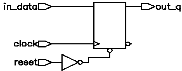
Figure 4-2 D Flip-Flop With an Active-High Asynchronous Reset
