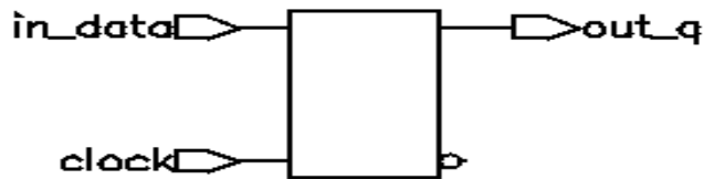
Figure 4-10 D Latch Inferred From an if Statement
