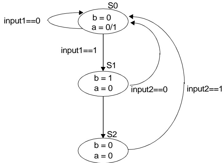
Figure 4-27 Finite State Machine State Diagram
