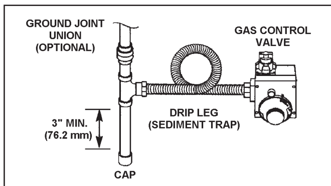
FIGURE 20. GAS PIPING WITH FLEXIBLE CONNECTOR.
