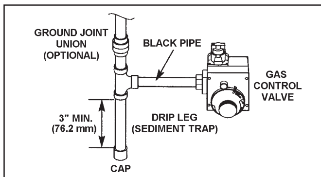
FIGURE 21. GAS PIPING WITH ALL BLACK IRON PIPE TO GAS CONTROL.
