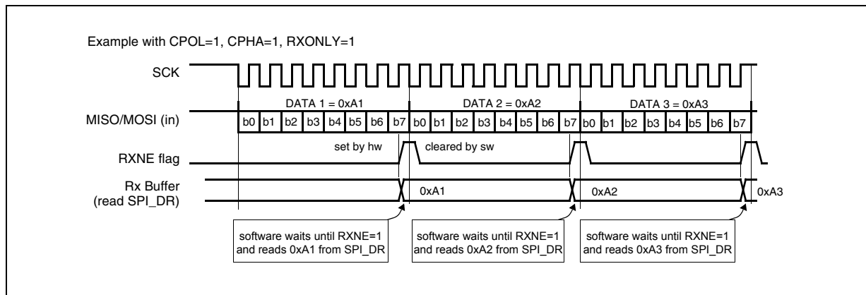
Figure 180. RXNE behavior in receive-only mode (BDM = 0 and RXONLY = 1). Case of continuous transfers
