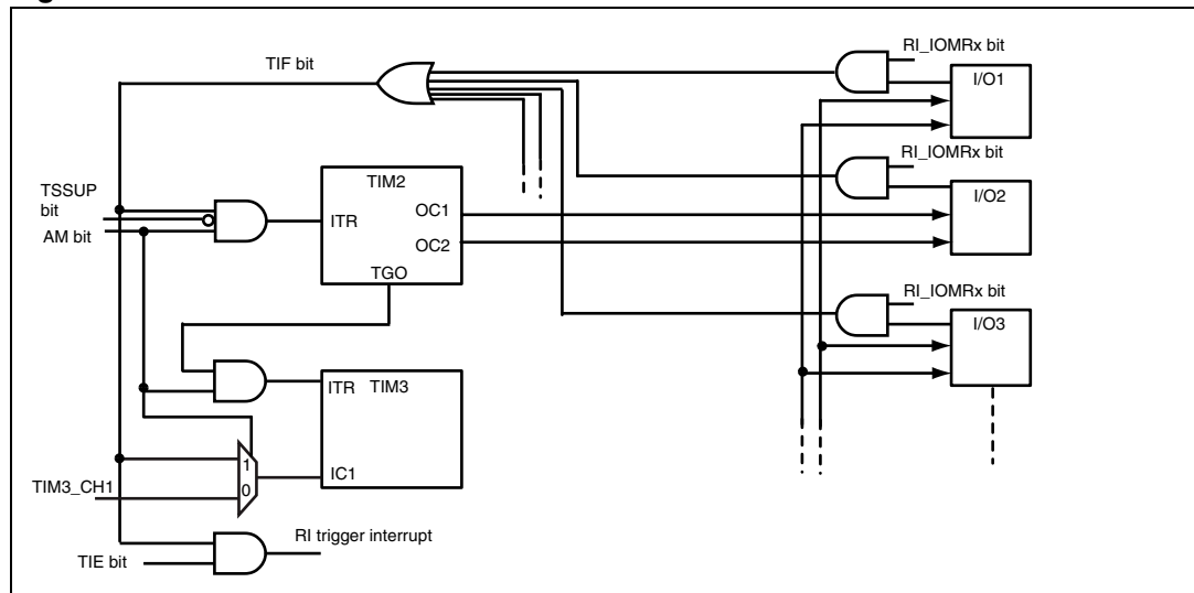
Figure 25. TIM2 and TIM3 interconnections
