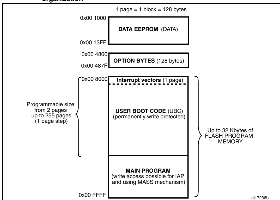
Figure 4. Medium density STM8L15xx Flash program and data EEPROM organization
