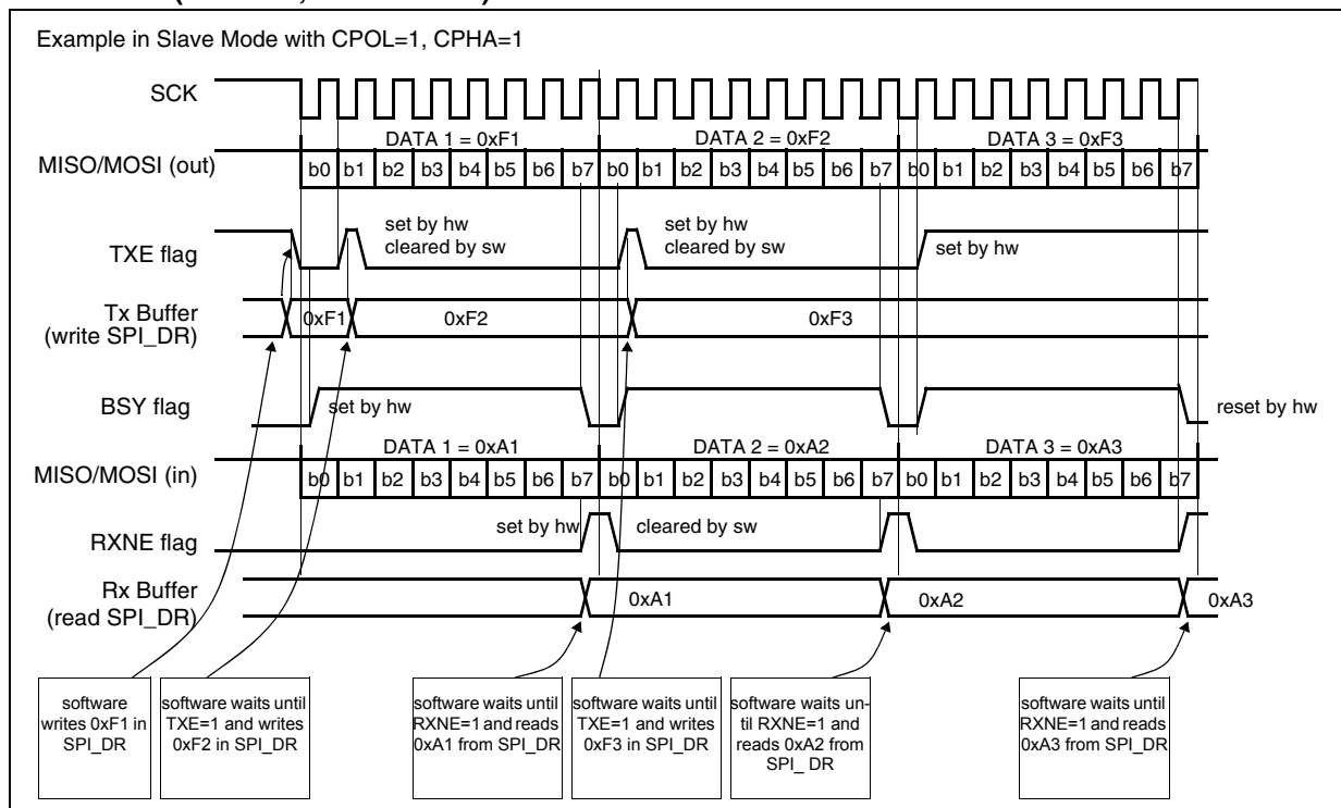
Figure 177. TXE/RXNE/BSY behavior in slave / full duplex mode (BDM = 0, RXONLY = 0). Case of continuous transfers
