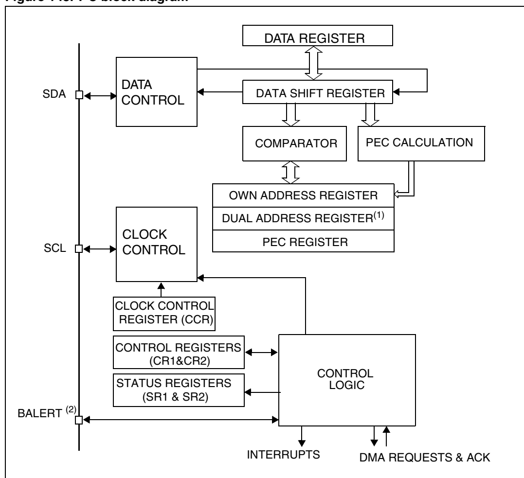
Figure 143. I 2 C block diagram
