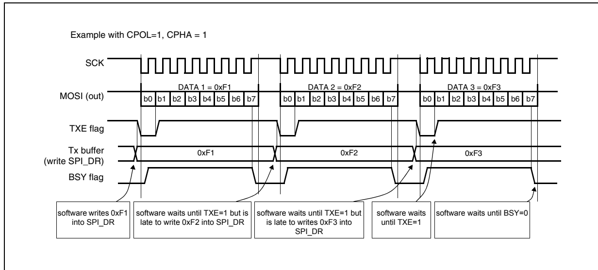
Figure 181. TXE/BSY behavior when transmitting (BDM = 0 and RXLON = 0). Case of discontinuous transfers
