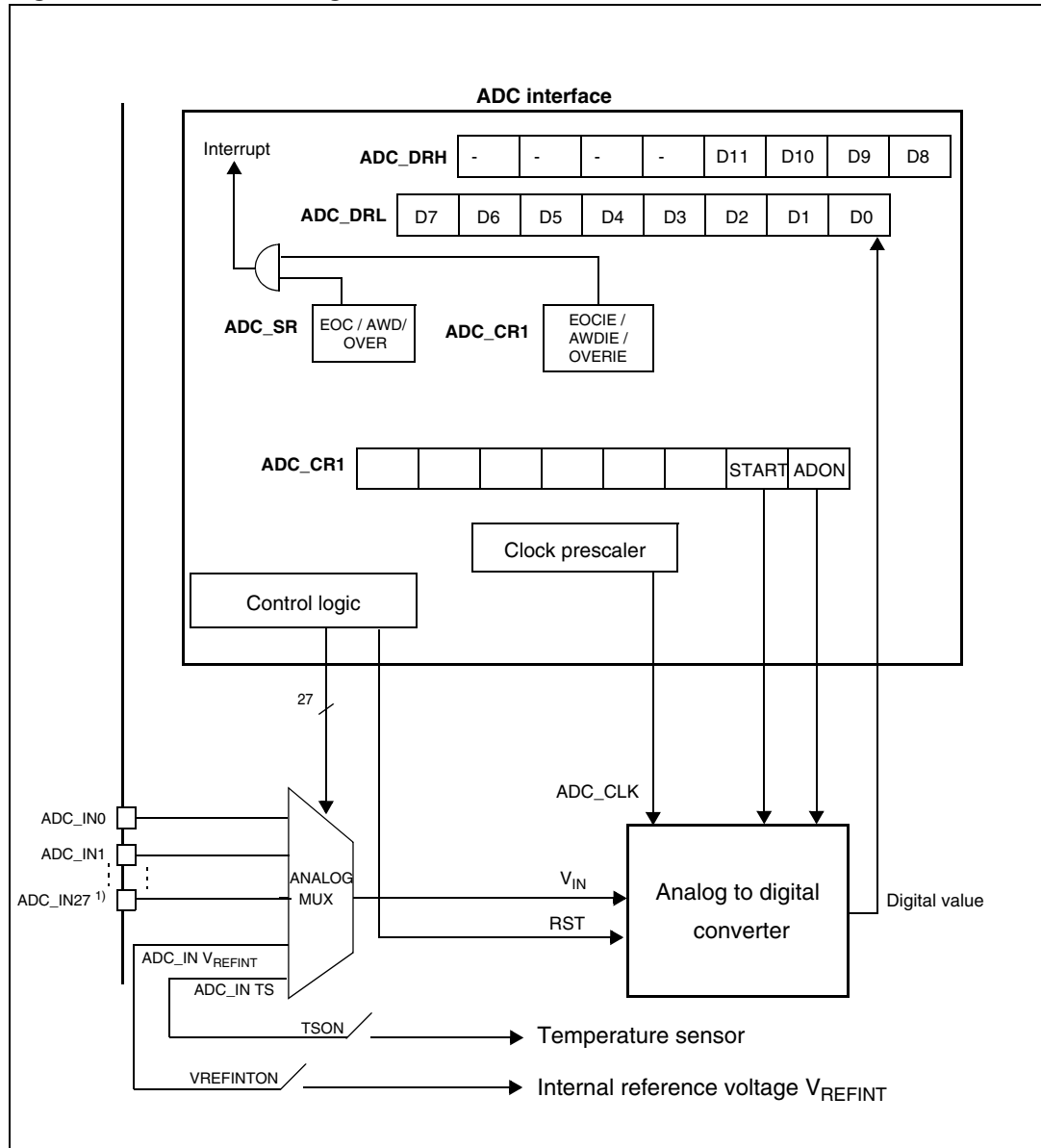
Figure 42. ADC block diagram
