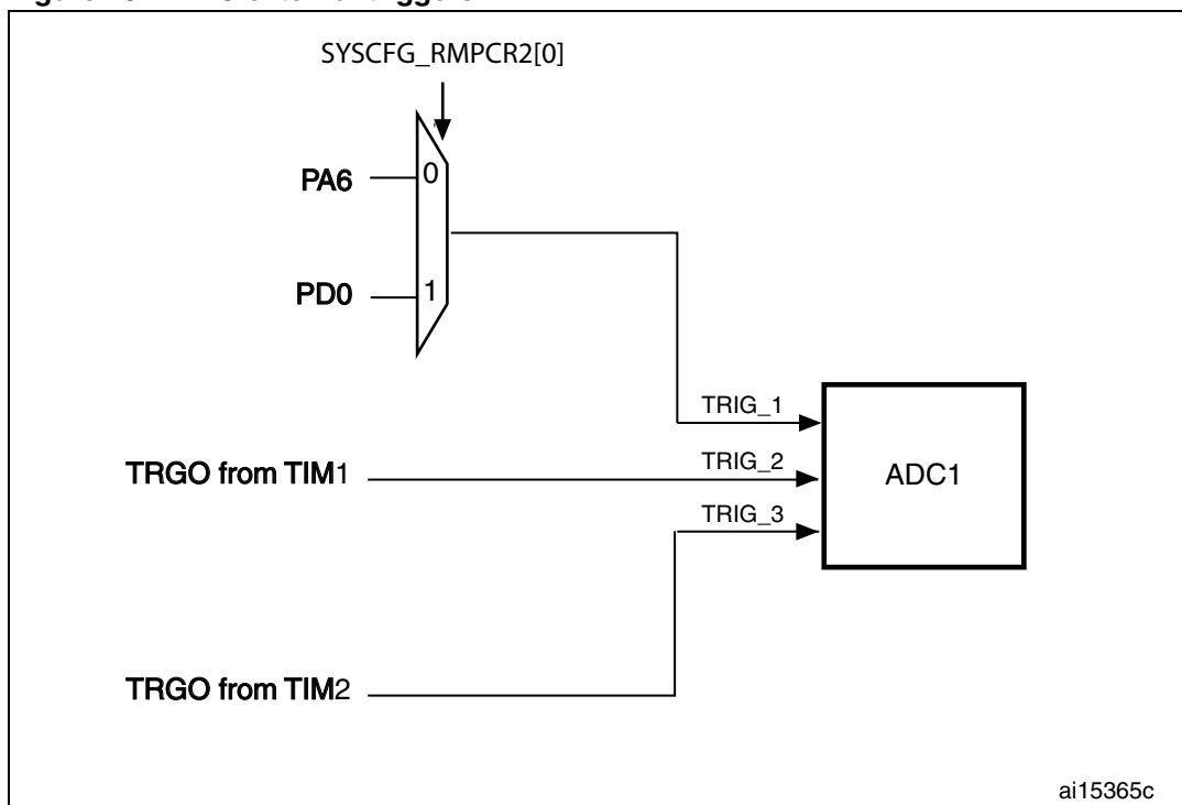
Figure 43. ADC external triggers
