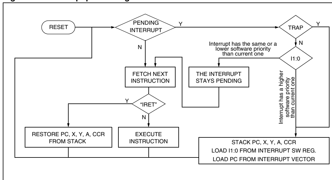
Figure 28. Interrupt processing flowchart
