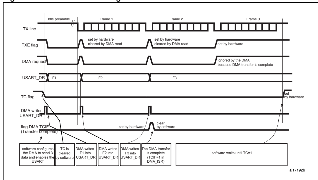
Figure 169. Transmission using DMA
