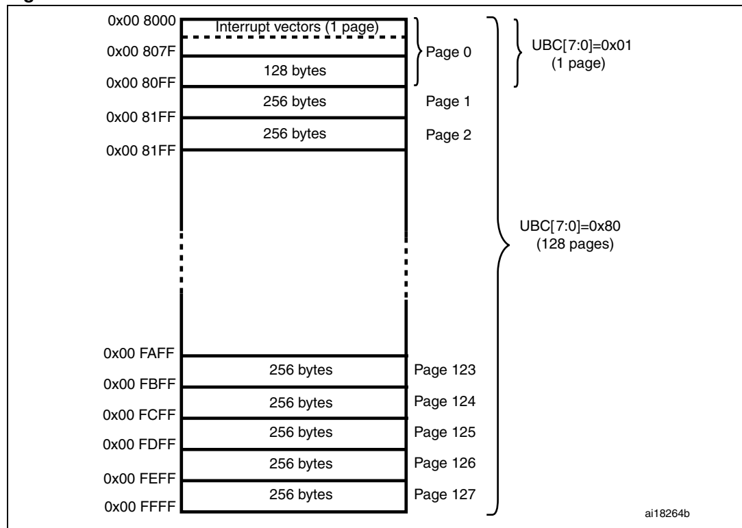
Figure 9. UBC area size definition for medium + STM8L15xx devices
