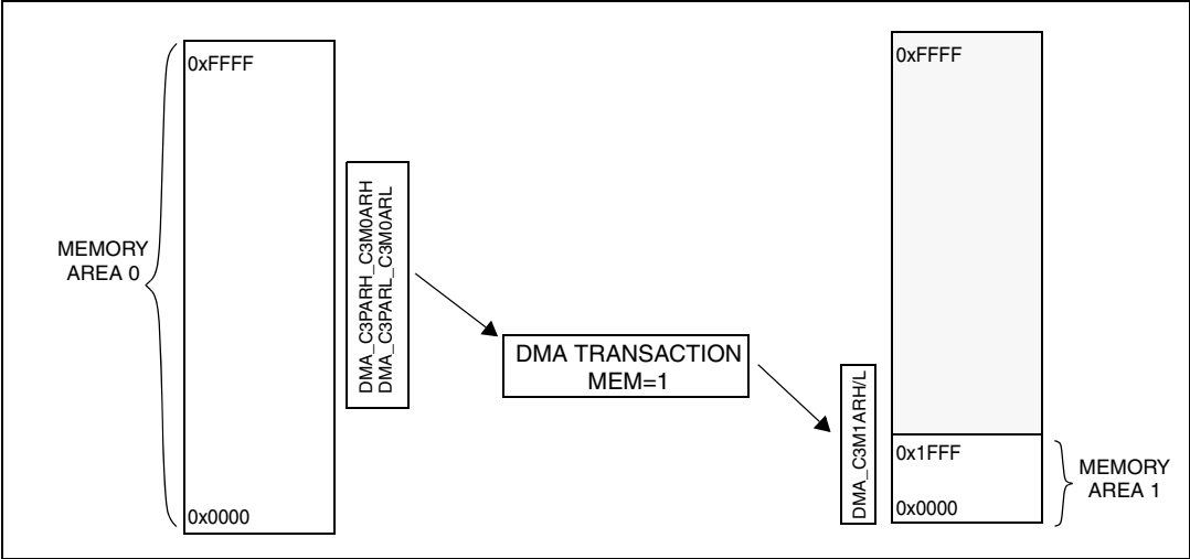
Figure 38. Memory channel with MEM=1 (medium density devices)
