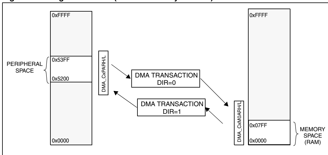
Figure 34. Regular channel (medium density devices)
