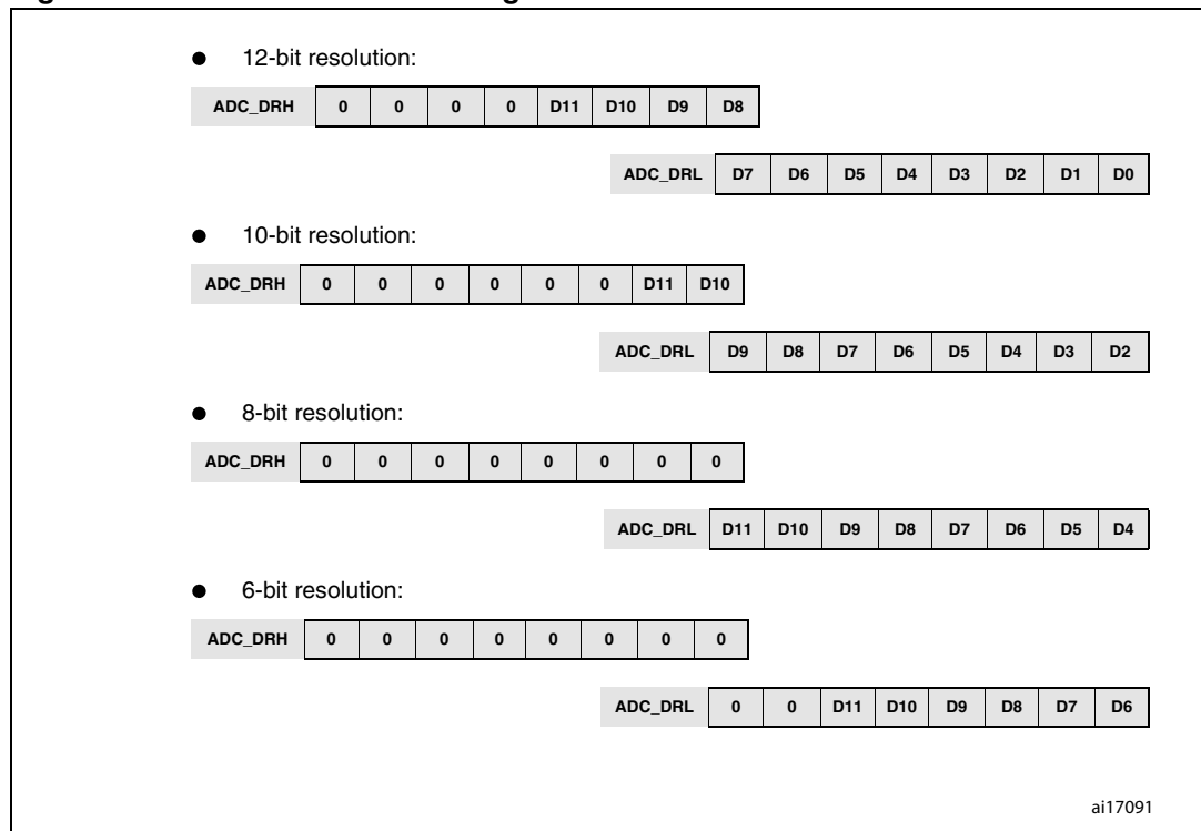
Figure 45. Resolution and data alignment
