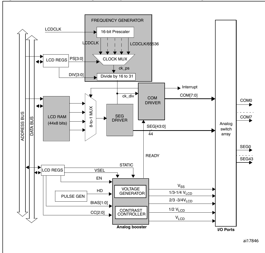
Figure 55. Medium + and high density LCD controller block diagram
