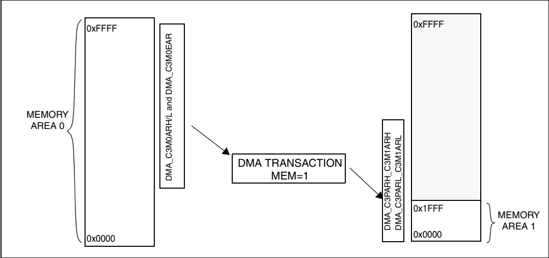
Figure 39. Memory channel with MEM=1 (medium+ and high density devices)
