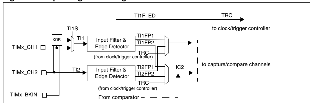
Figure 123. Input stage of TIM 2 channel 1
