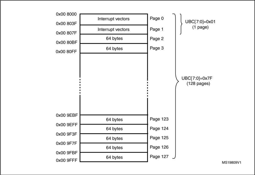
Figure 8. UBC area size definition for medium density STM8L15xx devices
