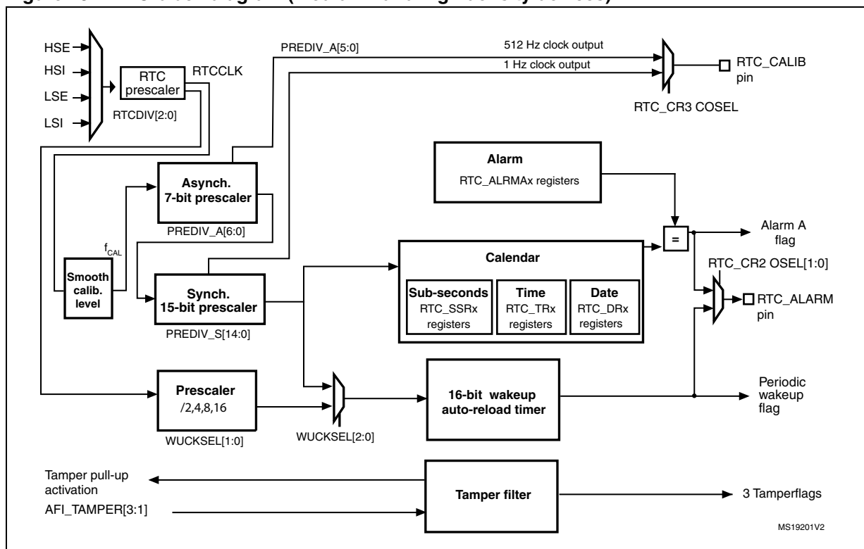
Figure 131. RTC block diagram (medium+ and high density devices)
