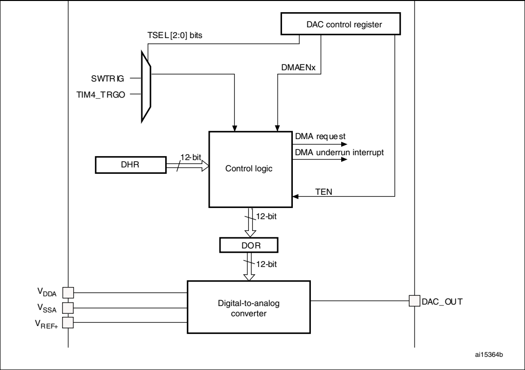
Figure 46. DAC channel block diagram (medium density devices)
