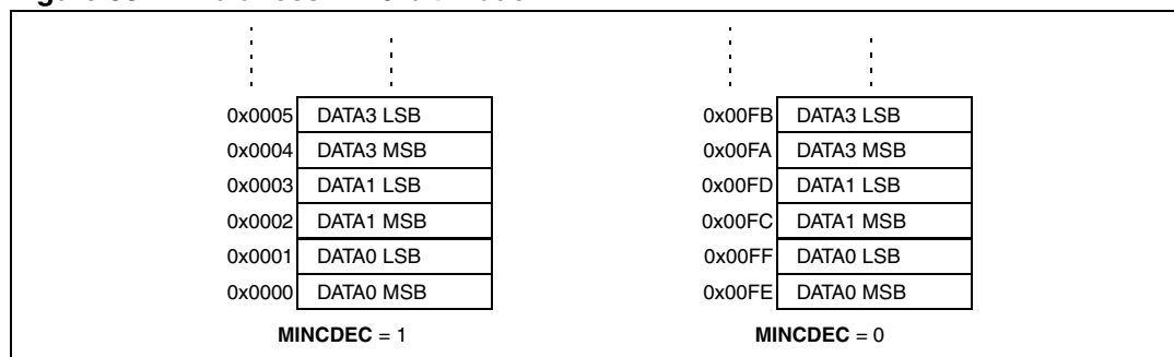
Figure 33. Endianness in 16-bit mode
