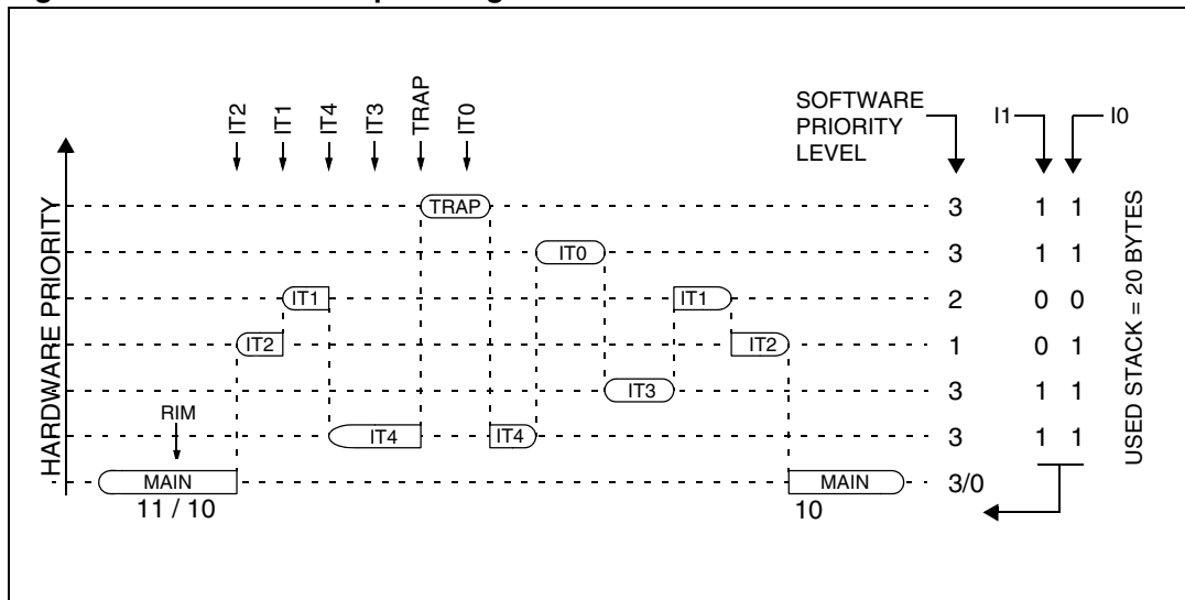
Figure 31. Nested interrupt management
