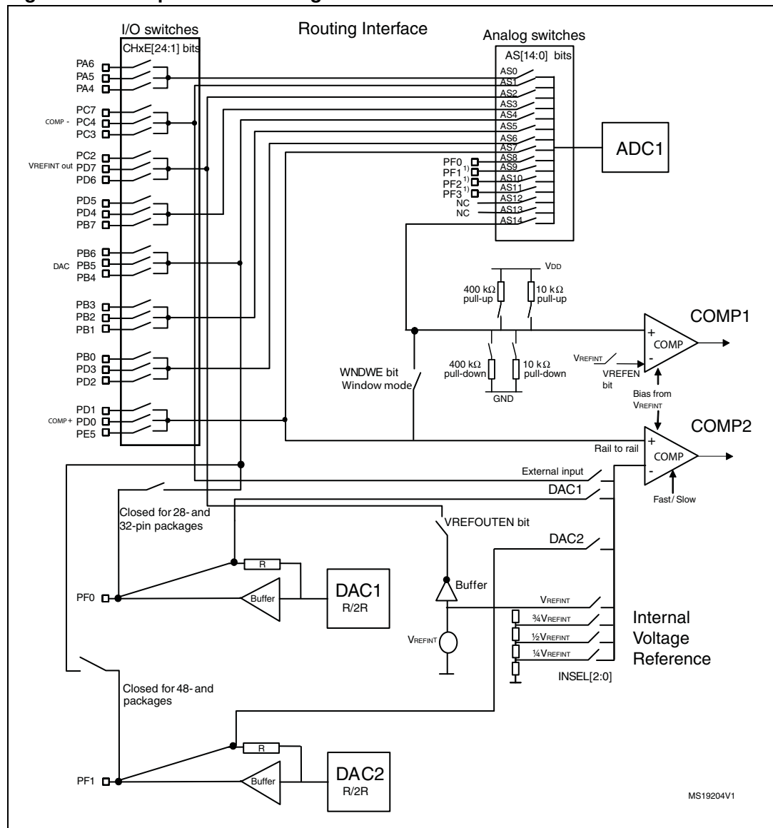
Figure 50. Comparator block diagram
