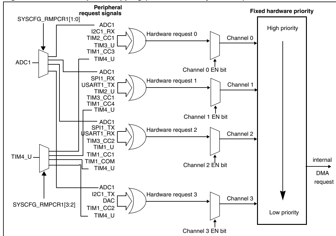
Figure 40. DMA1 request mapping (medium density devices)
