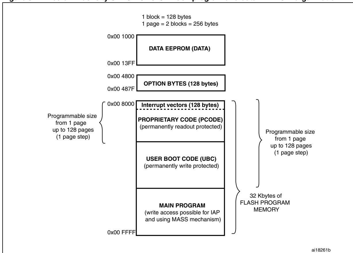
Figure 5. Medium+ density STM8L15xx/16x Flash program and data EEPROM organization
