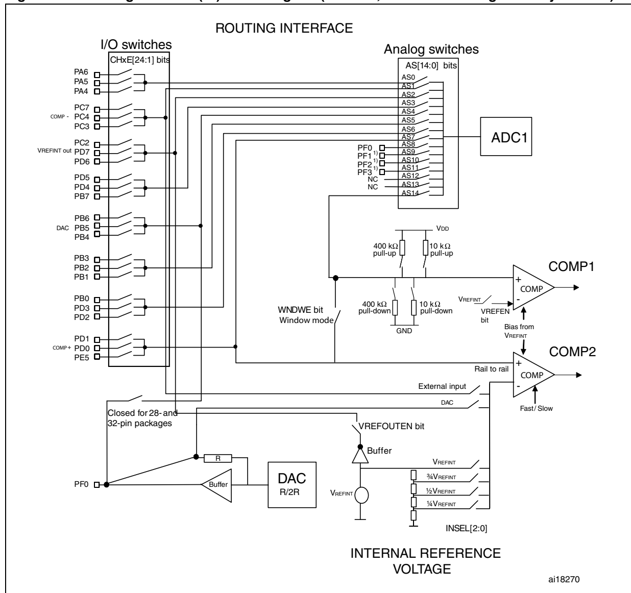
Figure 23. Routing interface (RI) block diagram (medium, medium+ and high density devices)
