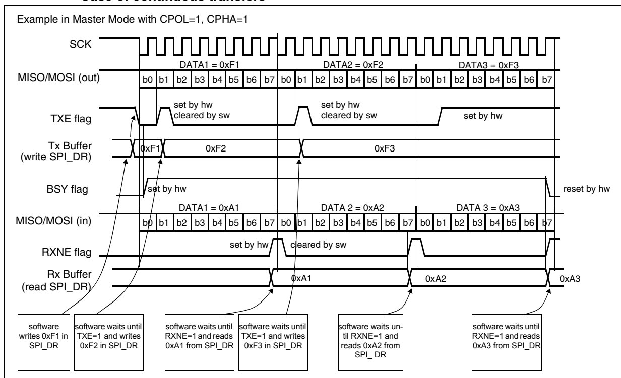
Figure 176. TXE/RXNE/BSY behavior in full duplex mode (RXONLY = 0). Case of continuous transfers
