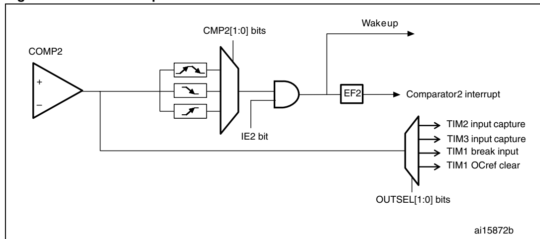
Figure 53. COMP2 output redirection
