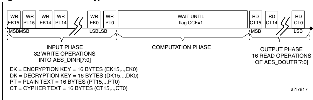
Figure 136. Mode 1: encryption
