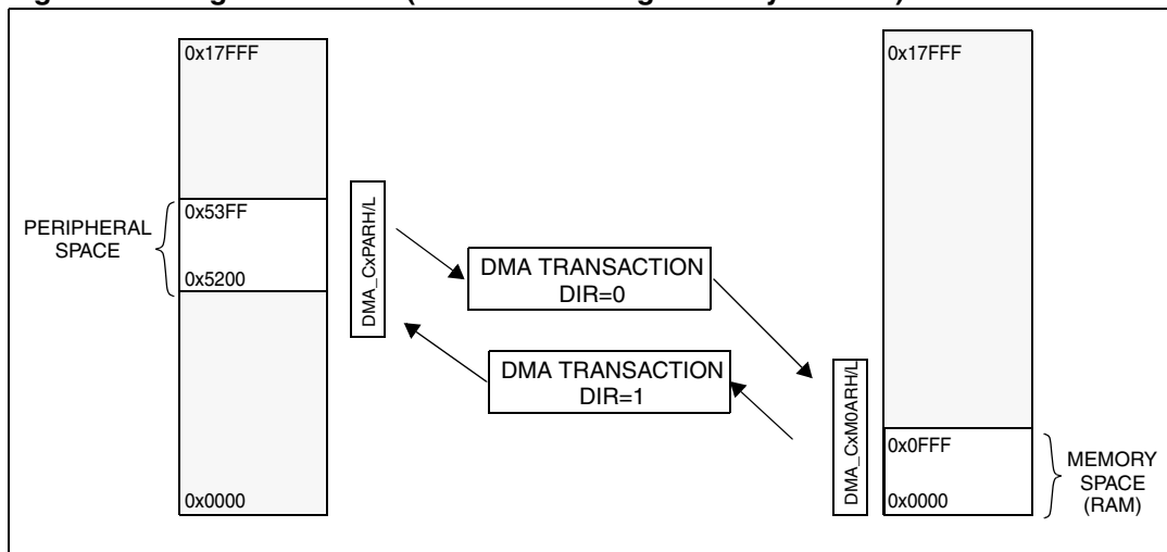
Figure 35. Regular channel (medium+ and high density devices)
