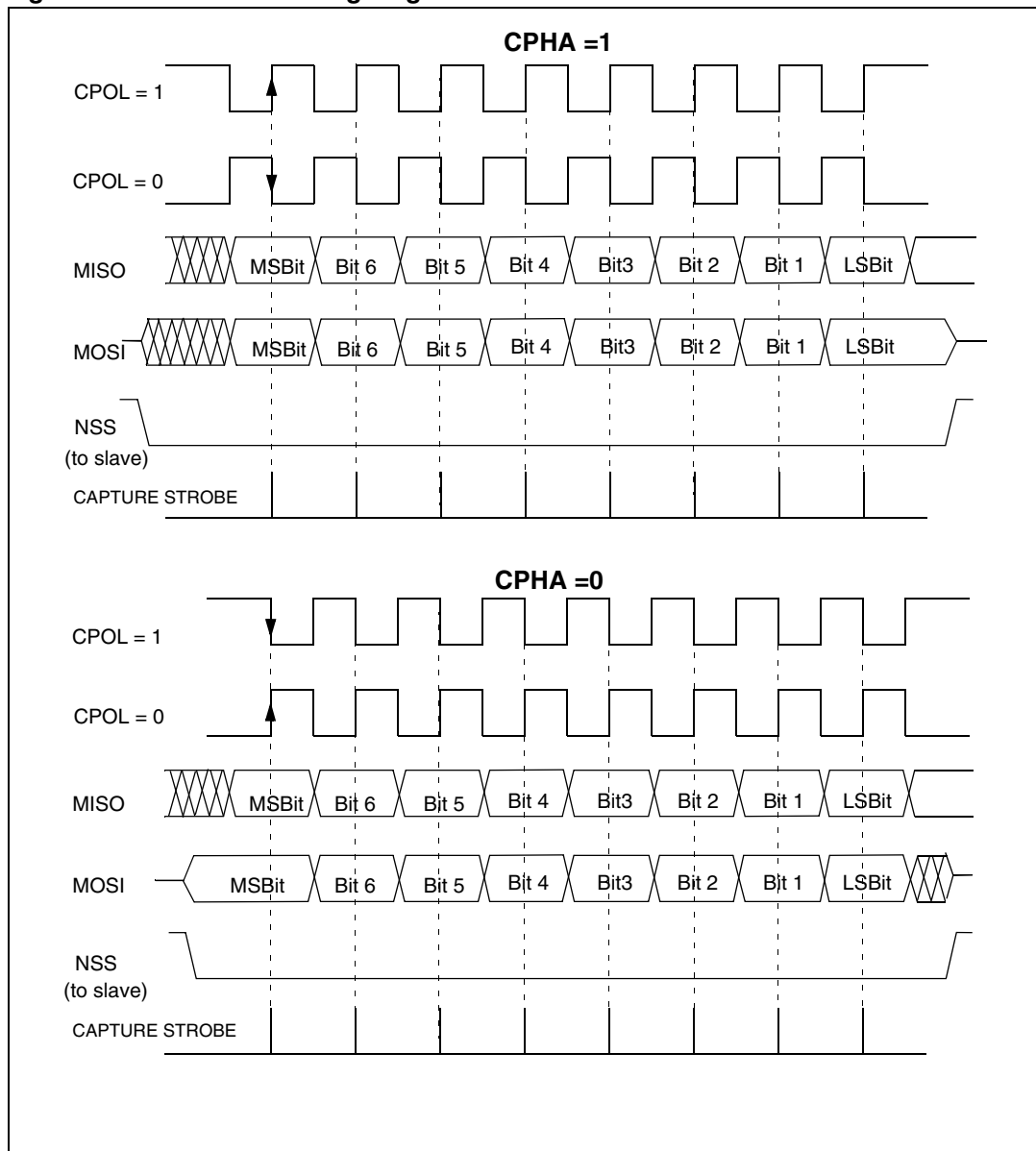
Figure 175. Data clock timing diagram
