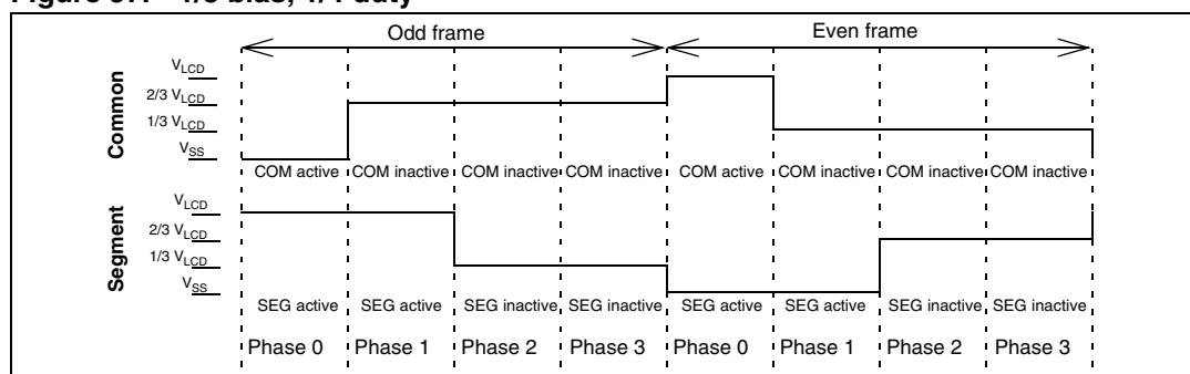
Figure 57. 1/3 bias, 1/4 duty
