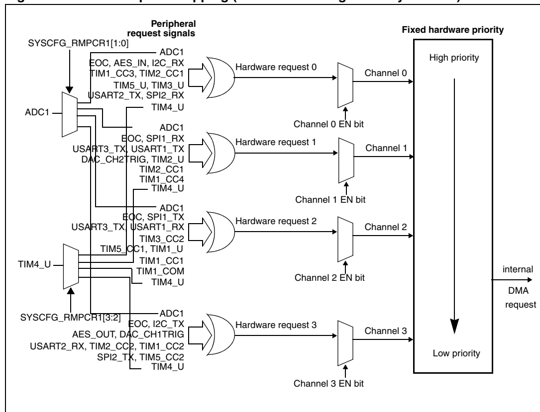
Figure 41. DMA1 request mapping (medium+ and high density devices)
