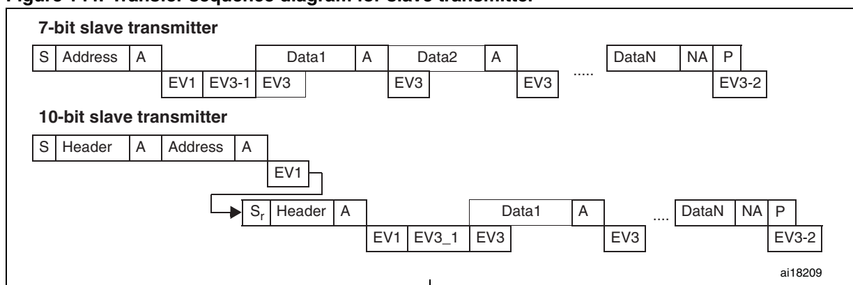
Figure 144. Transfer sequence diagram for slave transmitter
