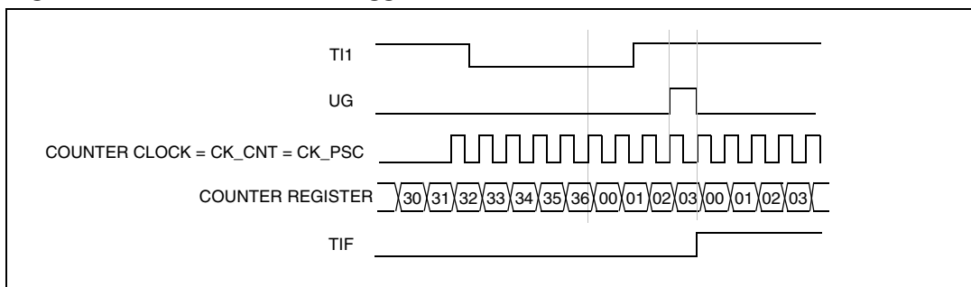
Figure 86. Control circuit in trigger reset mode
