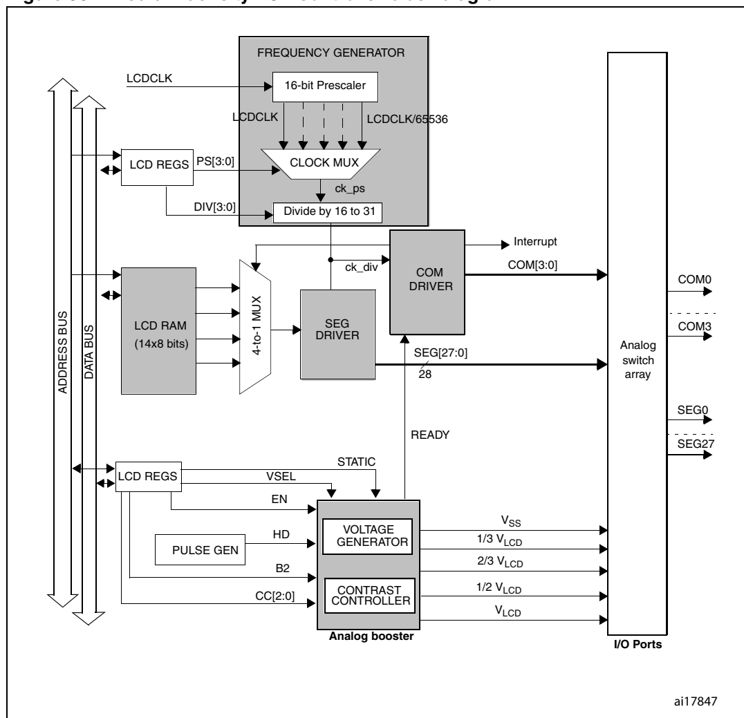
Figure 56. Medium density LCD controller block diagram
