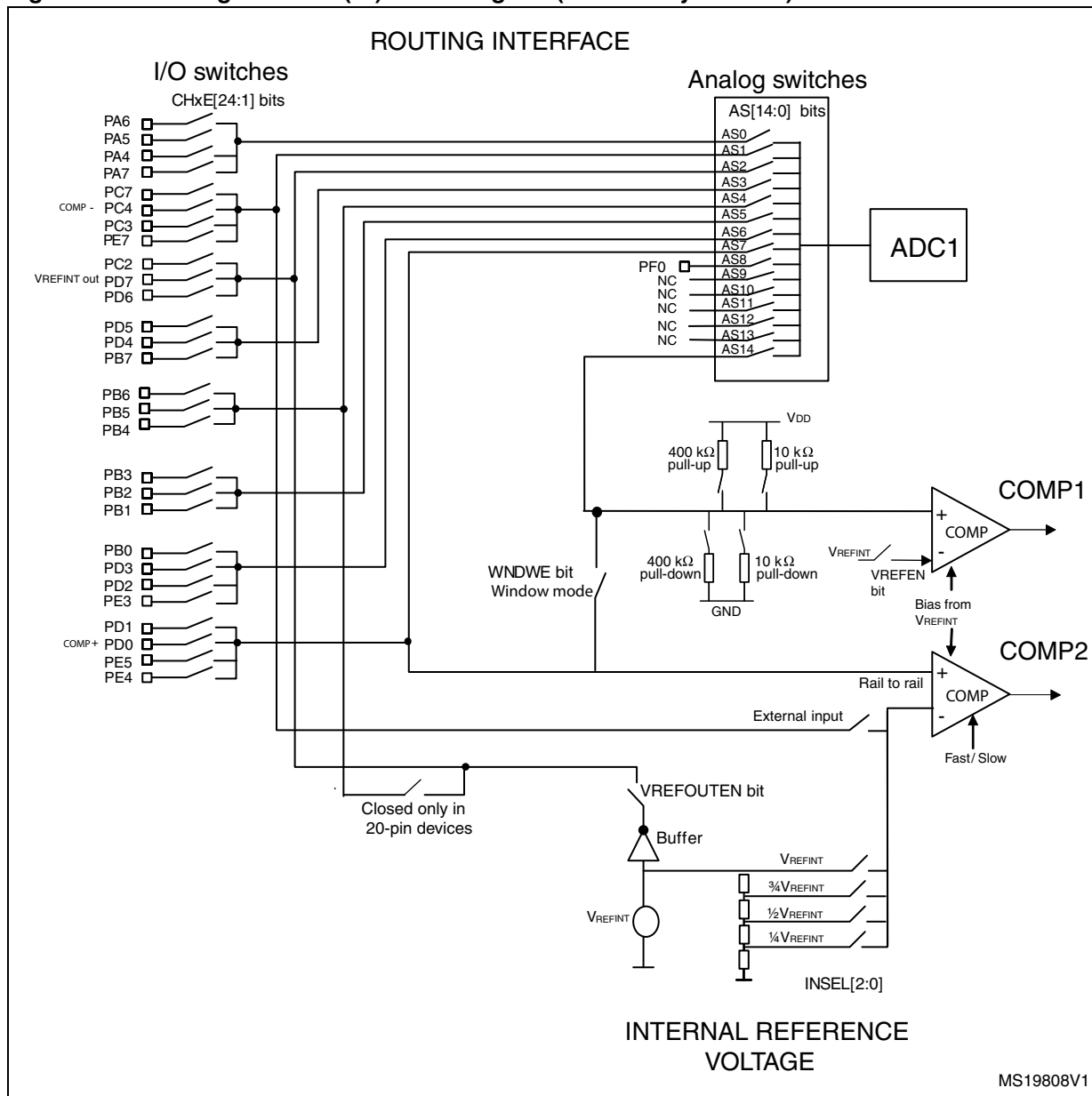
Figure 24. Routing interface (RI) block diagram (low density devices)
