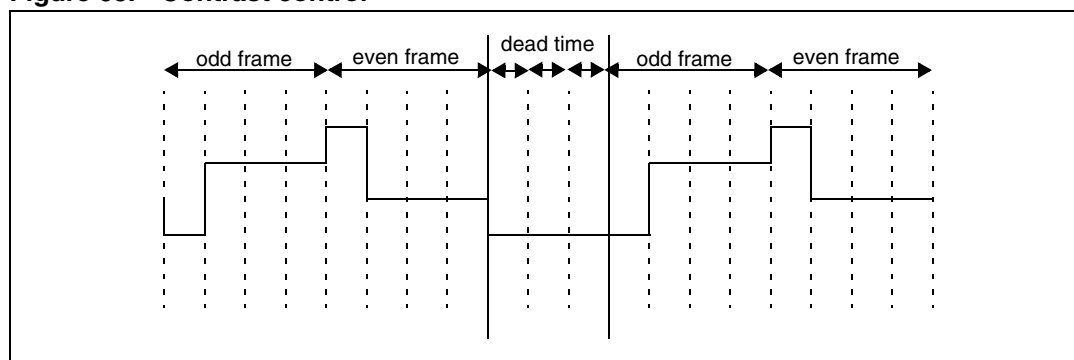
Figure 65. Contrast control
