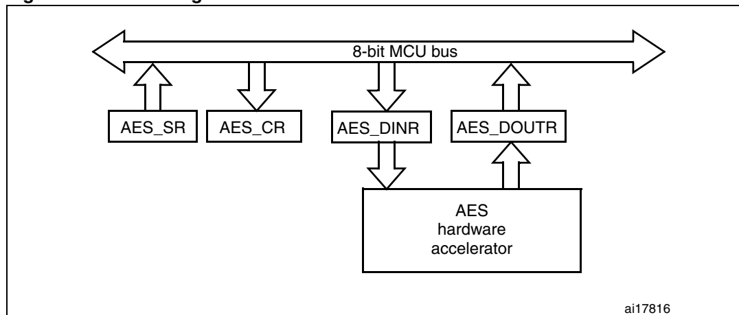
Figure 135. Block diagram
