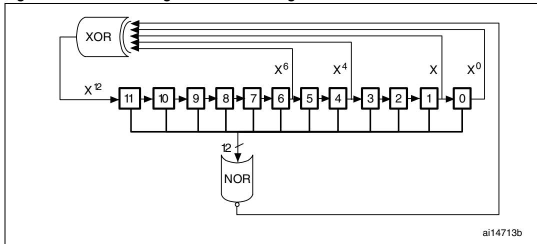
Figure 48. DAC LFSR register calculation algorithm
