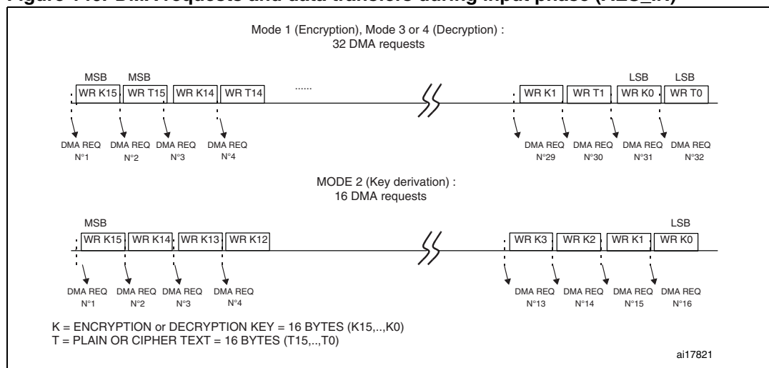
Figure 140. DMA requests and data transfers during input phase (AES_IN)
