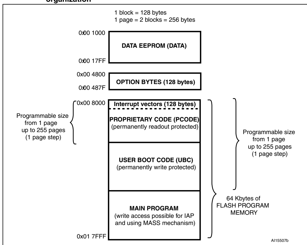
Figure 6. High density STM8L15xx/16x Flash program and data EEPROM organization
