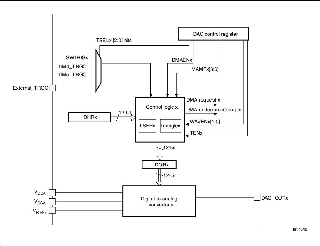
Figure 47. DAC channel block diagram (medium+ and high density devices)
