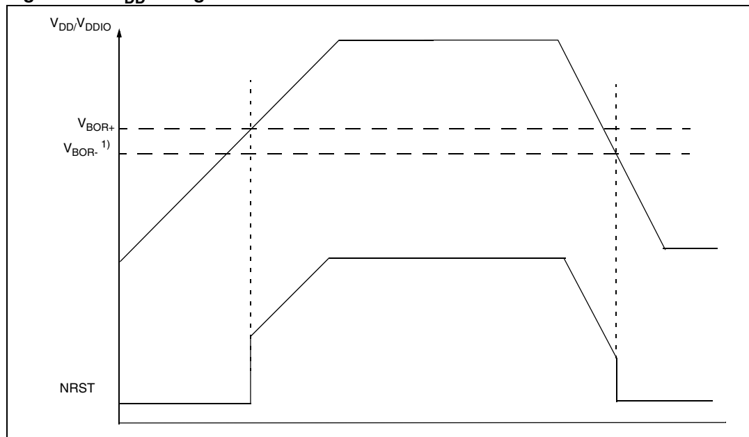
Figure 14. V_{DD} voltage detection: BOR threshold
