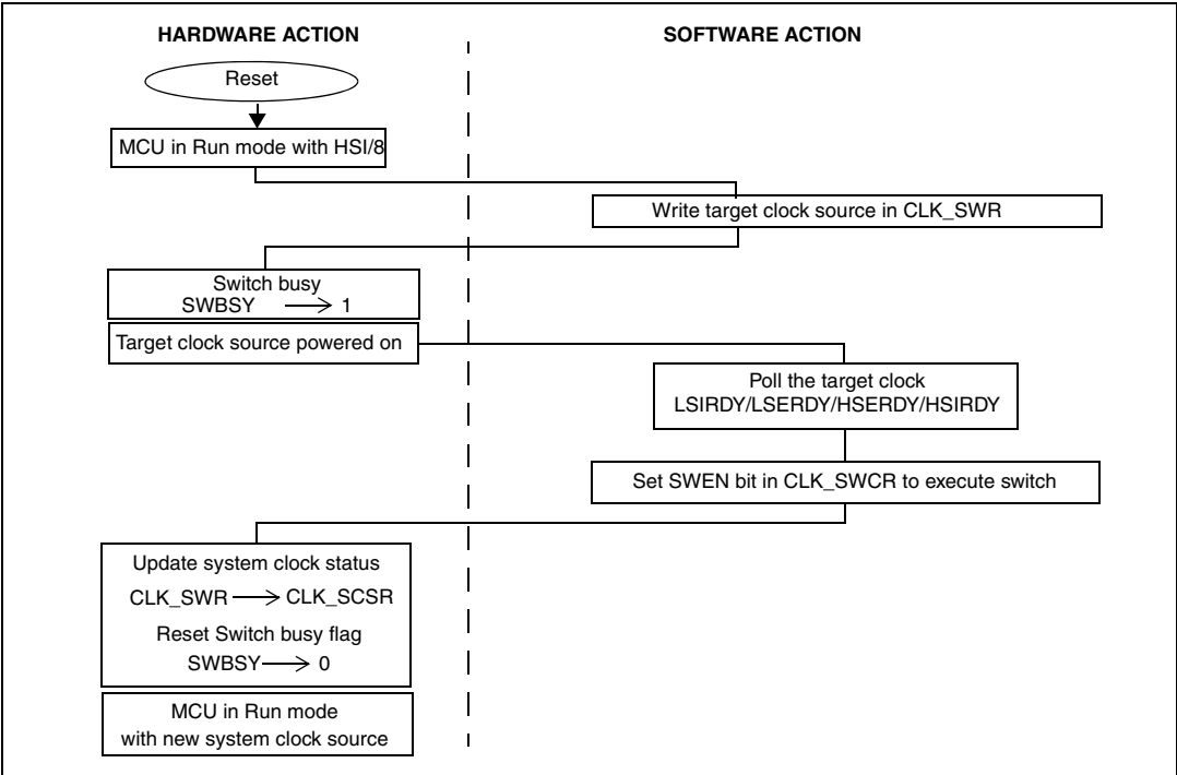
Figure 20. Clock switching flowchart (manual mode example without interrupt)
