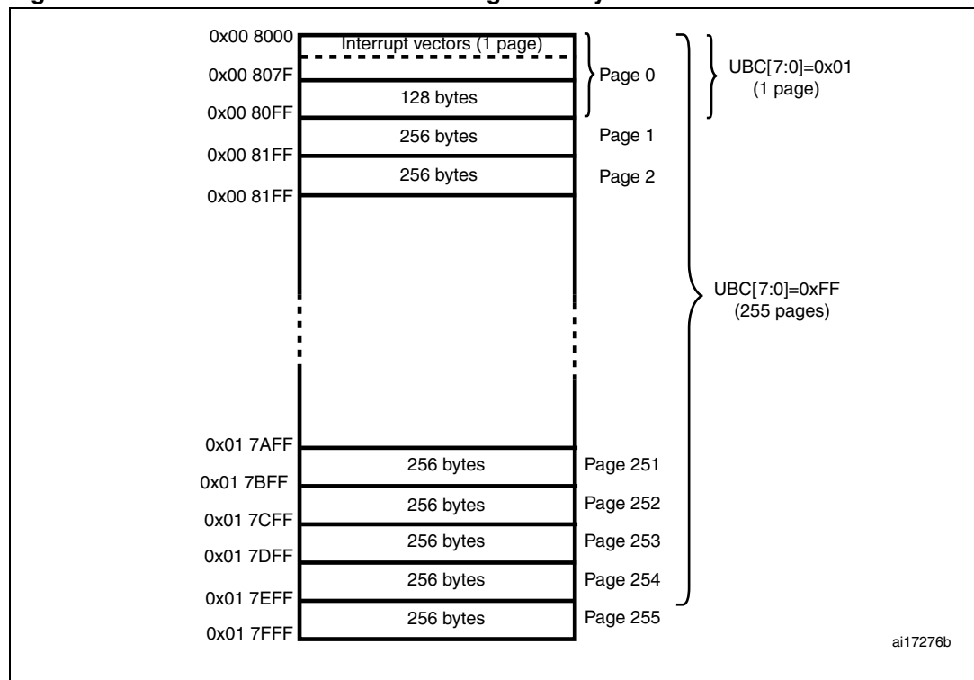
Figure 10. UBC area size definition for high density STM8L15xx/16x devices
