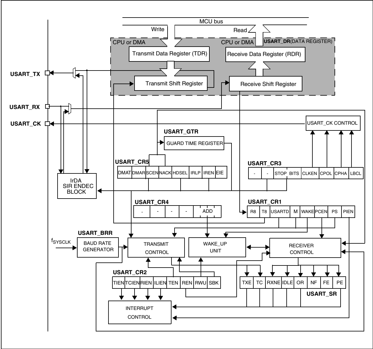
Figure 152. STM8L15xx USART block diagram
