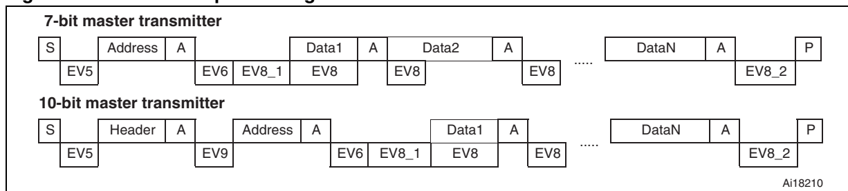
Figure 146. Transfer sequence diagram for master transmitter
