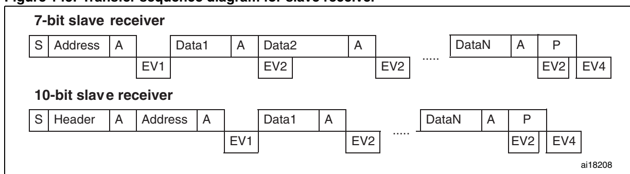
Figure 145. Transfer sequence diagram for slave receiver
