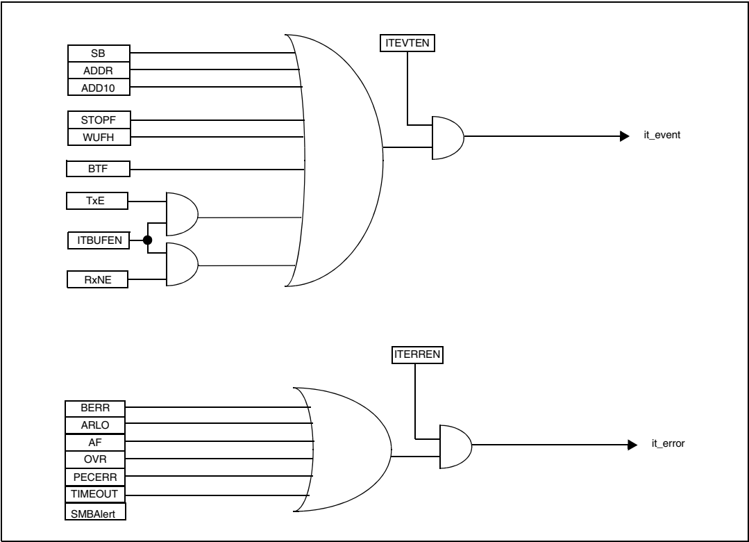
Figure 151. STM8L15xx I 2 C interrupt mapping diagram
