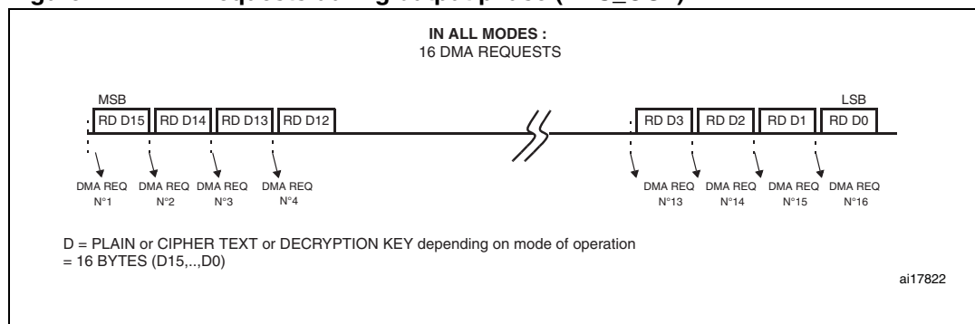
Figure 141. DMA requests during output phase (AES_OUT)
