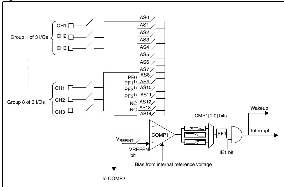
Figure 51. COMP1 interconnections
