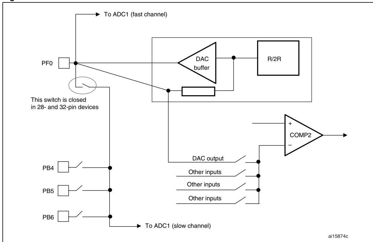
Figure 26. DAC interconnections
