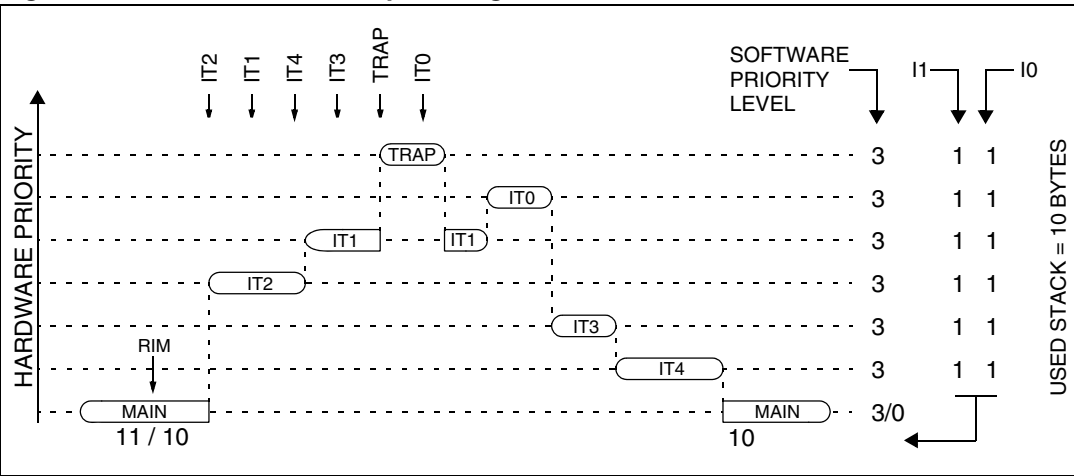
Figure 30. Concurrent interrupt management
