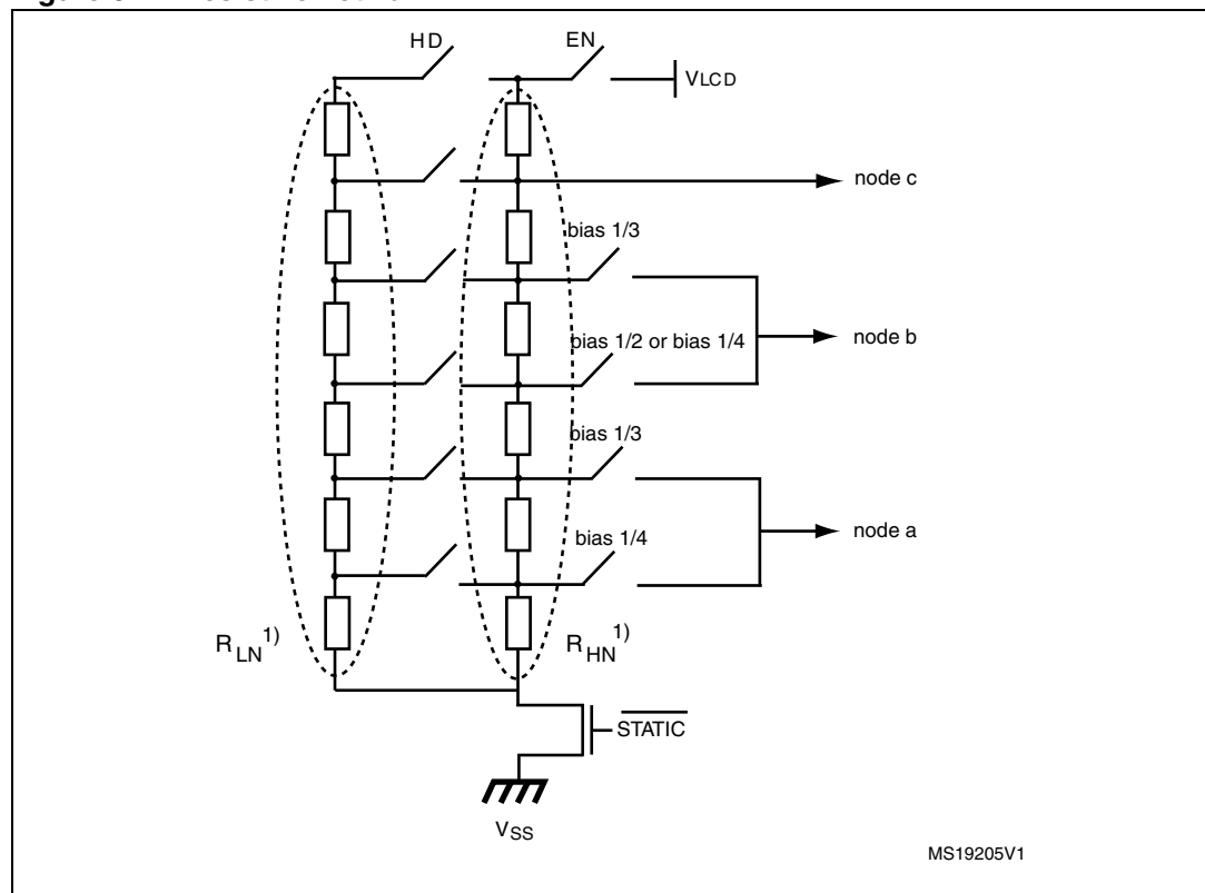
Figure 64. Resistive network
