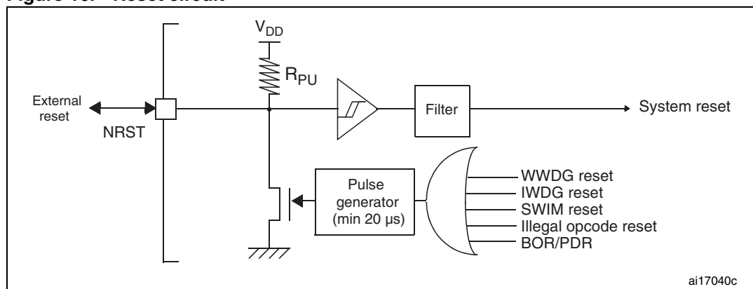
Figure 16. Reset circuit
