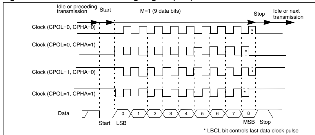
Figure 163. USART data clock timing diagram (M=1)
