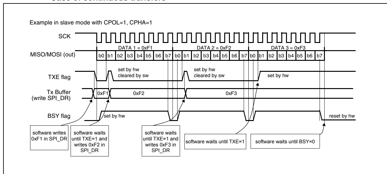
Figure 179. TXE/BSY in slave transmit-only mode (BDM = 0 and RXONLY = 0). Case of continuous transfers
