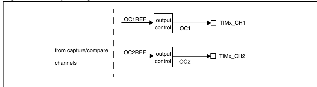
Figure 124. Output stage
