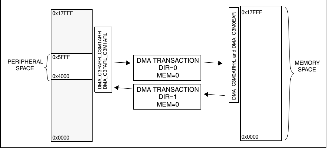
Figure 37. Memory channel with MEM=0 (medium+ and high density devices)
