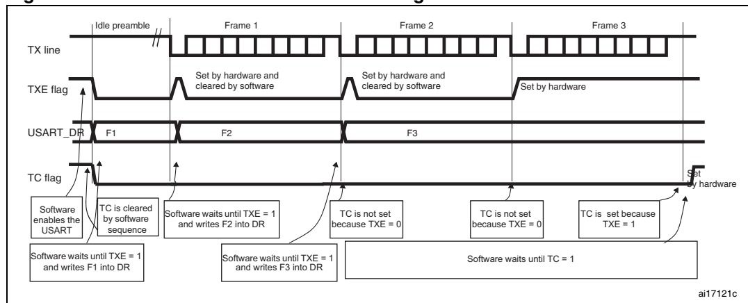
Figure 155. TC/TXE behavior when transmitting
