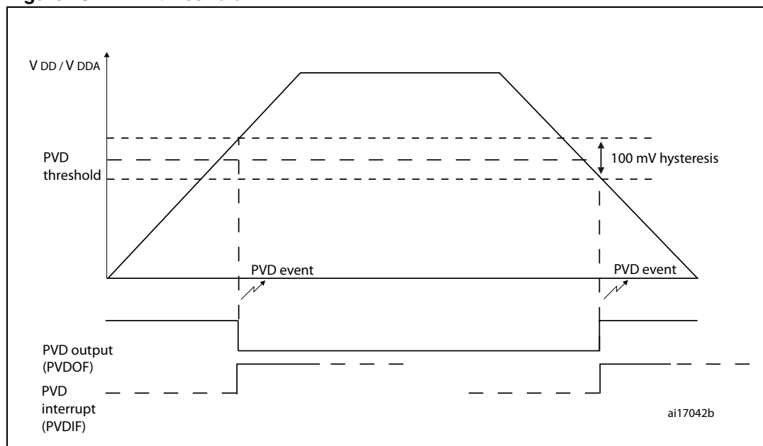
Figure 15. PVD threshold
