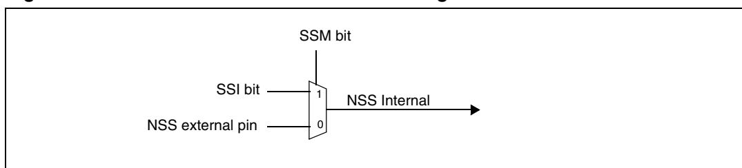
Figure 174. Hardware/software slave select management
