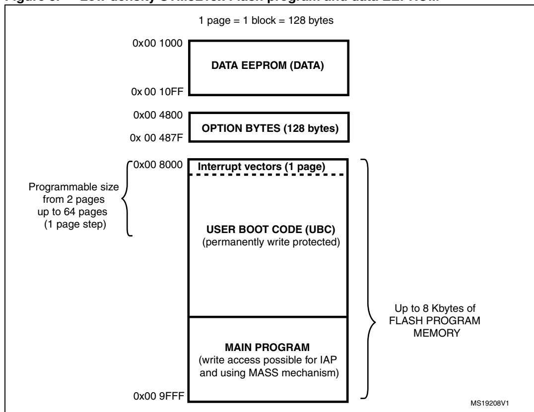
Figure 3. Low density STM8L15x Flash program and data EEPROM
