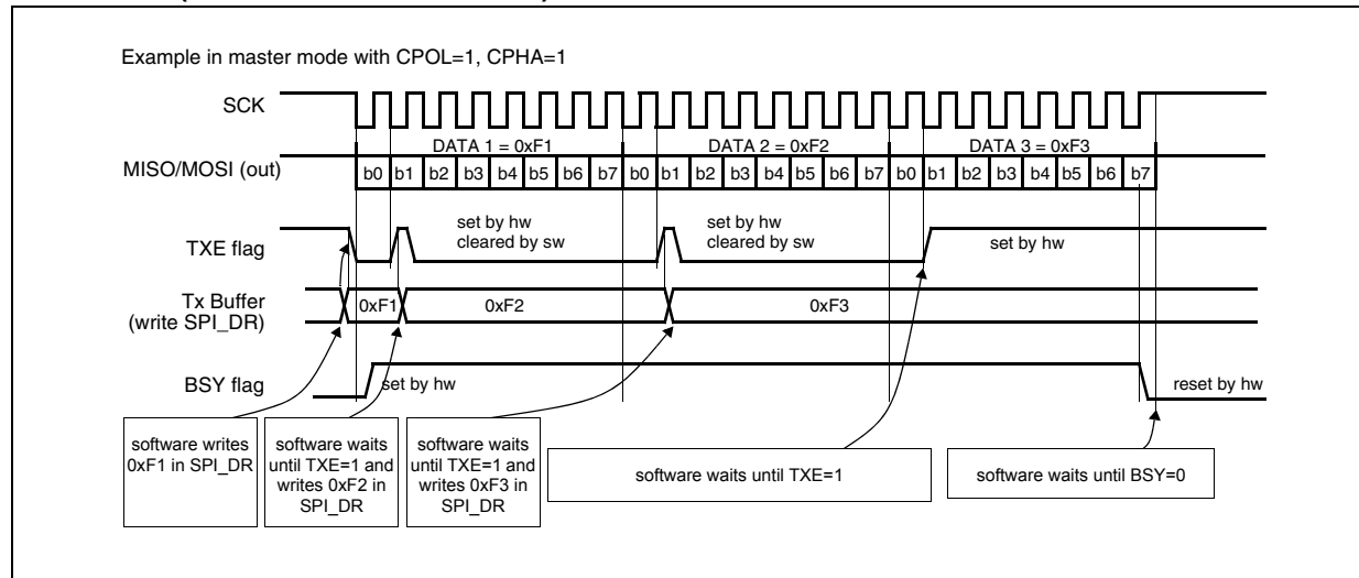
Figure 178. TXE/BSY in master transmit-only mode (BDM = 0 and RXONLY = 0). Case of continuous transfers
