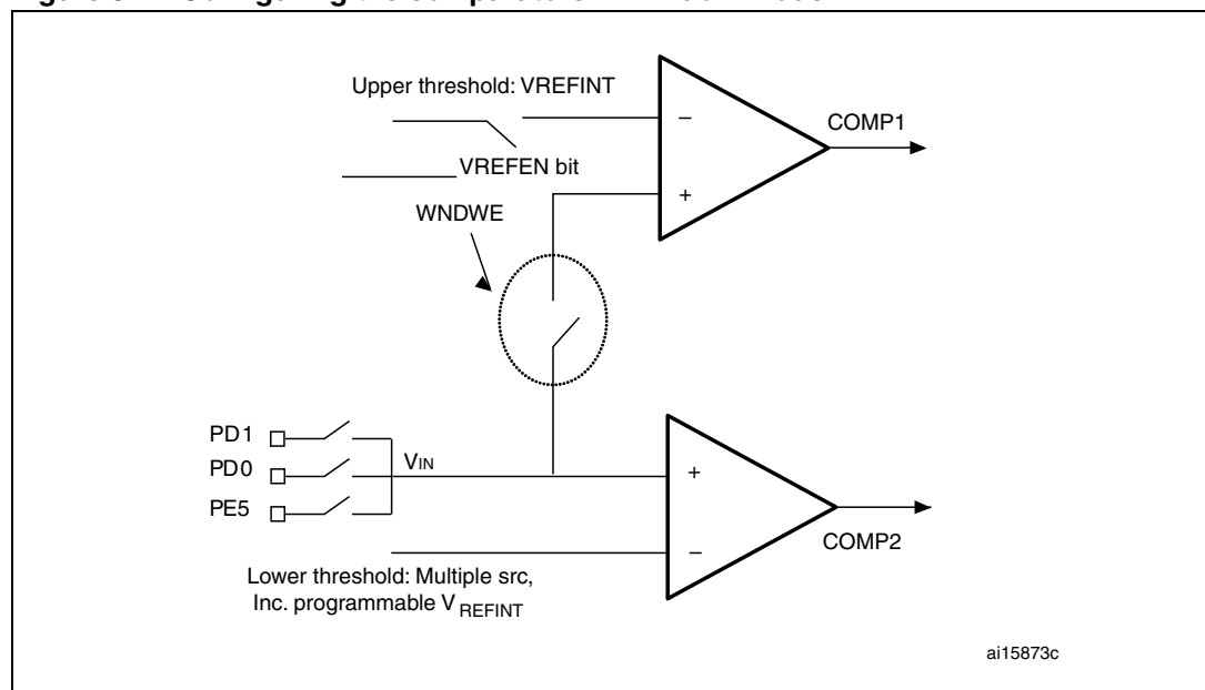
Figure 54. Configuring the comparators in window mode
