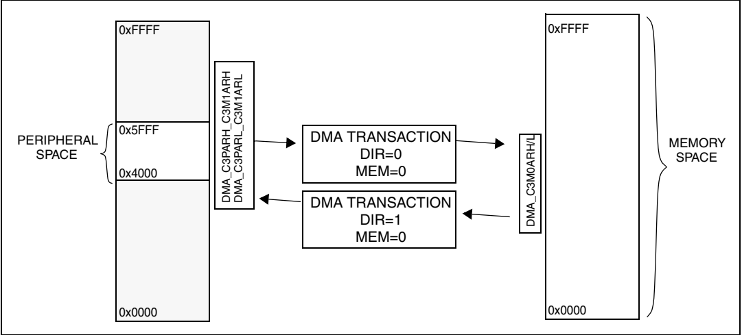
Figure 36. Memory channel with MEM=0 (medium density devices)
