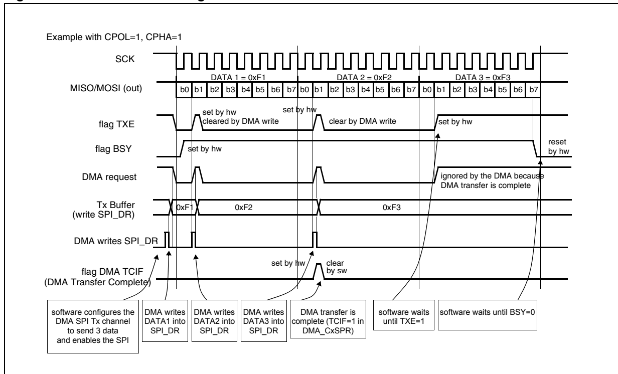
Figure 182. Transmission using DMA
