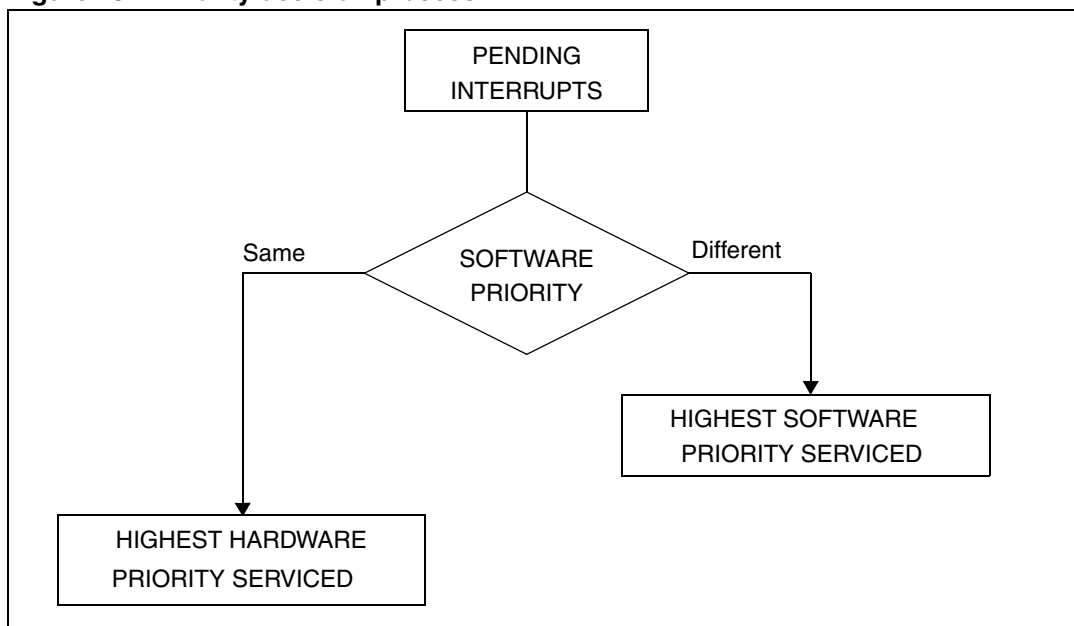
Figure 29. Priority decision process
