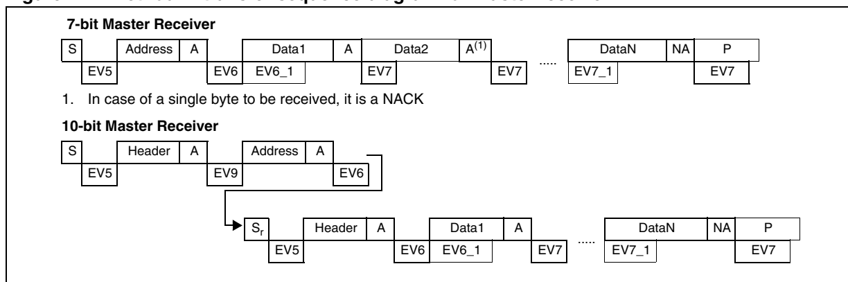
Figure 147. Method 1: transfer sequence diagram for master receiver
