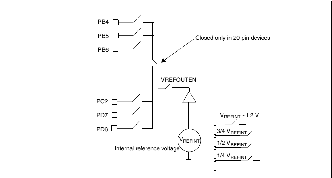
Figure 27. Internal reference voltage output
