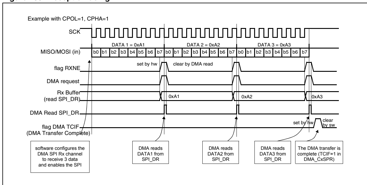
Figure 183. Reception using DMA
