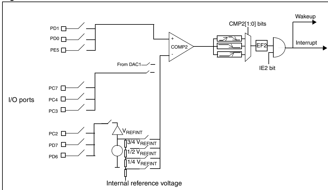
Figure 52. COMP2 interconnections
