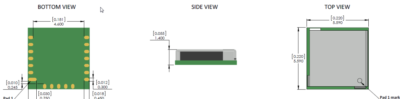
FIGURE 20 – MECHANICAL DRAWING
