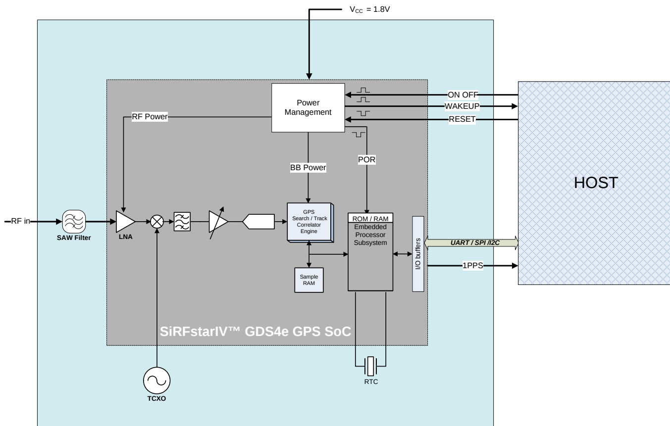
FIGURE 1 – ORG4475 ARCHITECTURE
