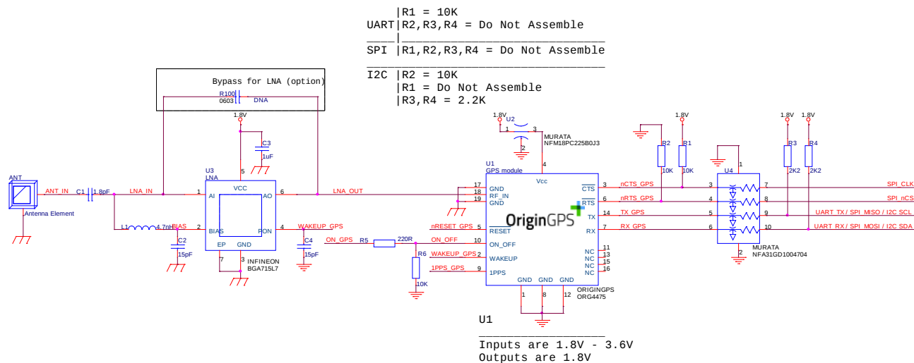
FIGURE 10 – SCHEMATIC DIAGRAM OF PASSIVE ANTENNA WITH EXTERNAL LNA
