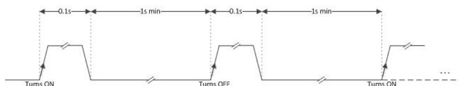
FIGURE 17 – ON_OFF TIMING
