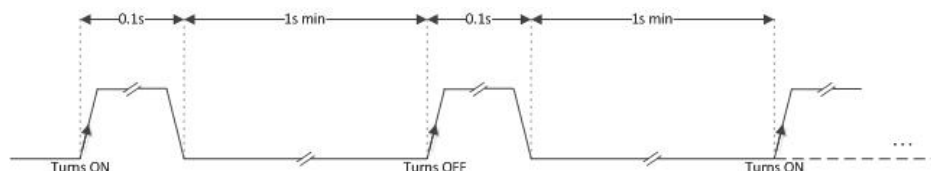
FIGURE 9 – ON_OFF TIMING
