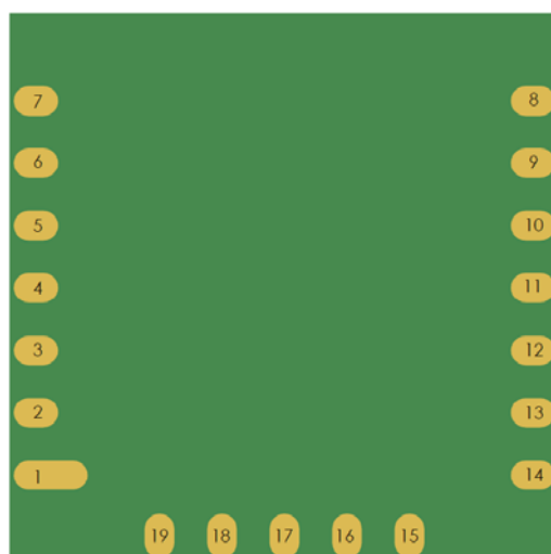
FIGURE 8 – PAD ASSIGNMENT
