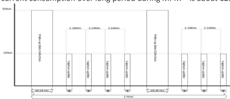
FIGURE 6 – MPM™ TIMING
