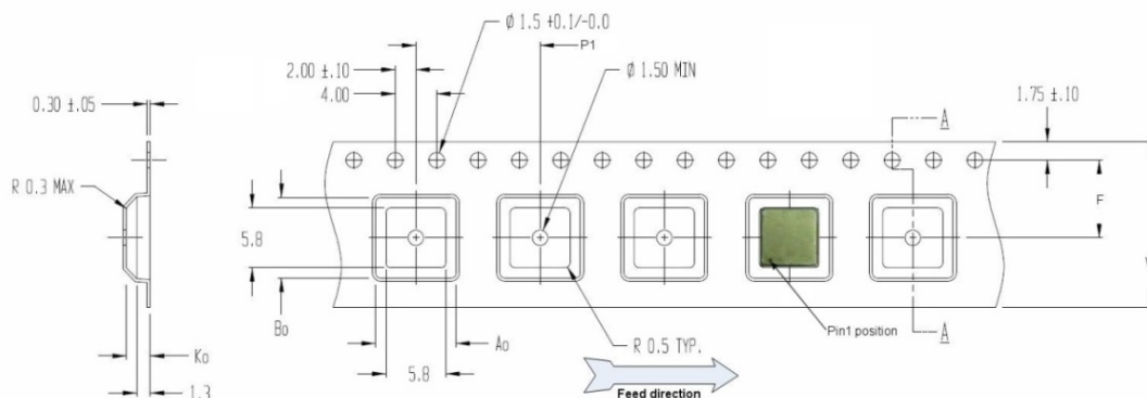
FIGURE 22 – CARRIER TAPE
