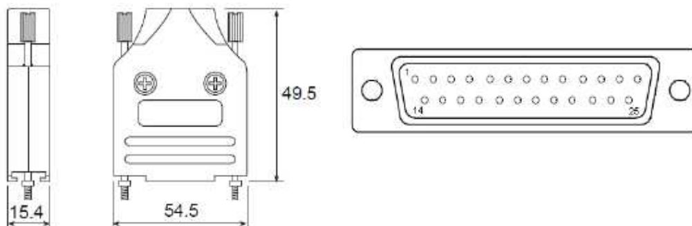
Figure 14: DB25 male connector (dimensions in millimeters)
