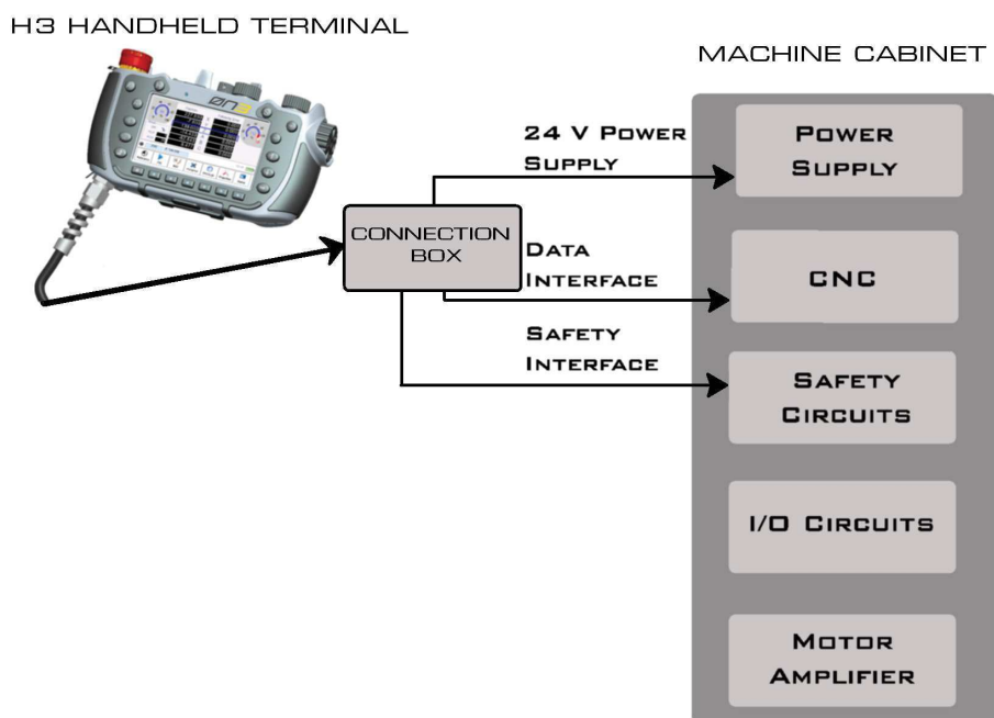
Figure 5: H3 system overview
