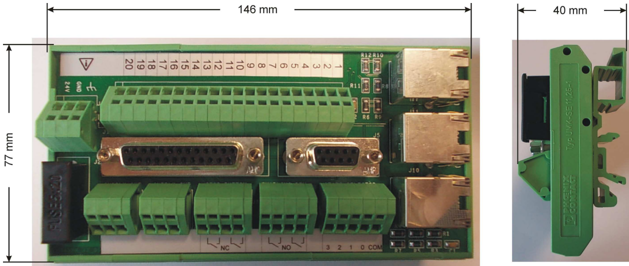
Figure 13: Connection Box dimensions
