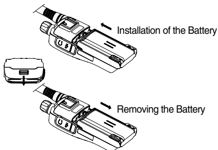
Figure 3-1) Installation and Removal of the Battery
