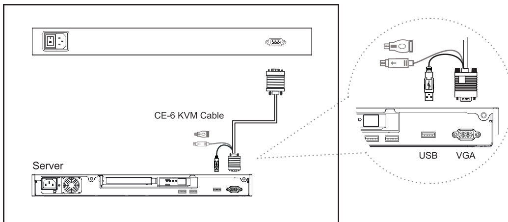
Figure 12. Example of connecting CE-6 4-in-1 Combo KVM cable to server via USB interface
