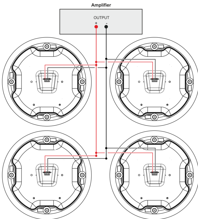
Figure 10: Square Layout Parallel Wiring
