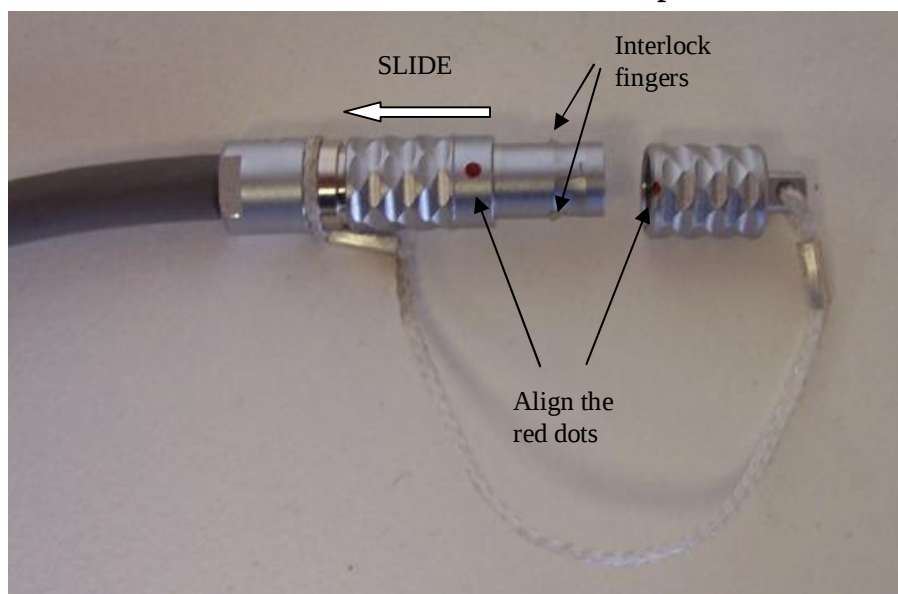
Figure 1a — Dust cap removal from probe cable
