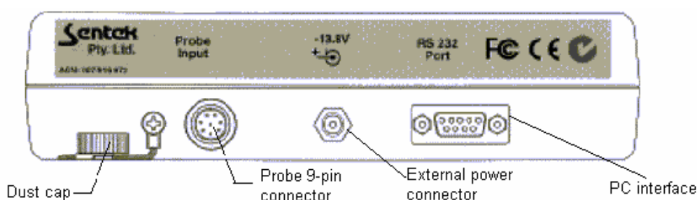
Figure 3—Connection Panel
