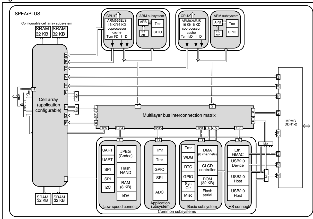
Figure 1. SPEAr600 architecture
