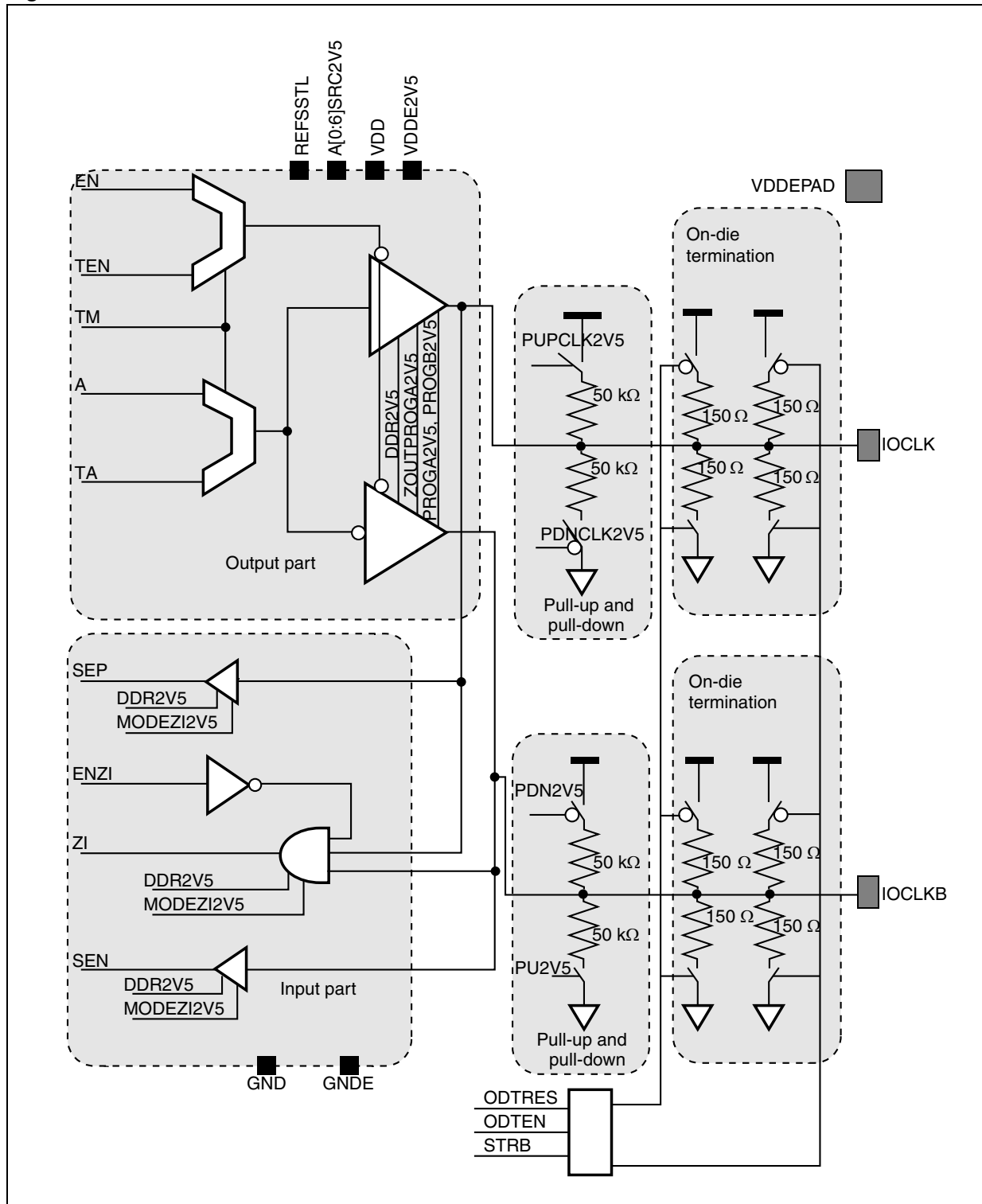
Figure 5. Clock cell
