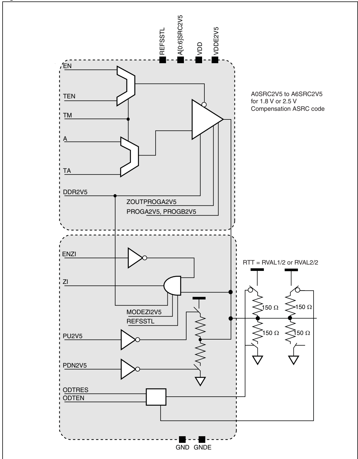
Figure 4. Data cell architecture
