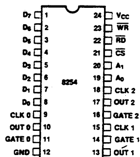
Figure 2. Pin Configuration
