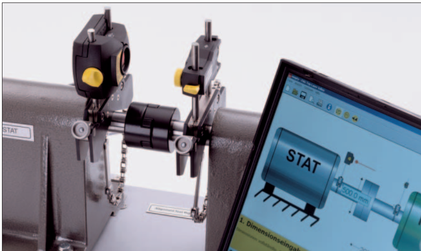
FAG Top-Laser INLINE in operation
