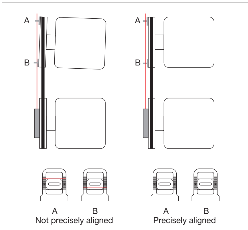
Alignment example using a belt drive
