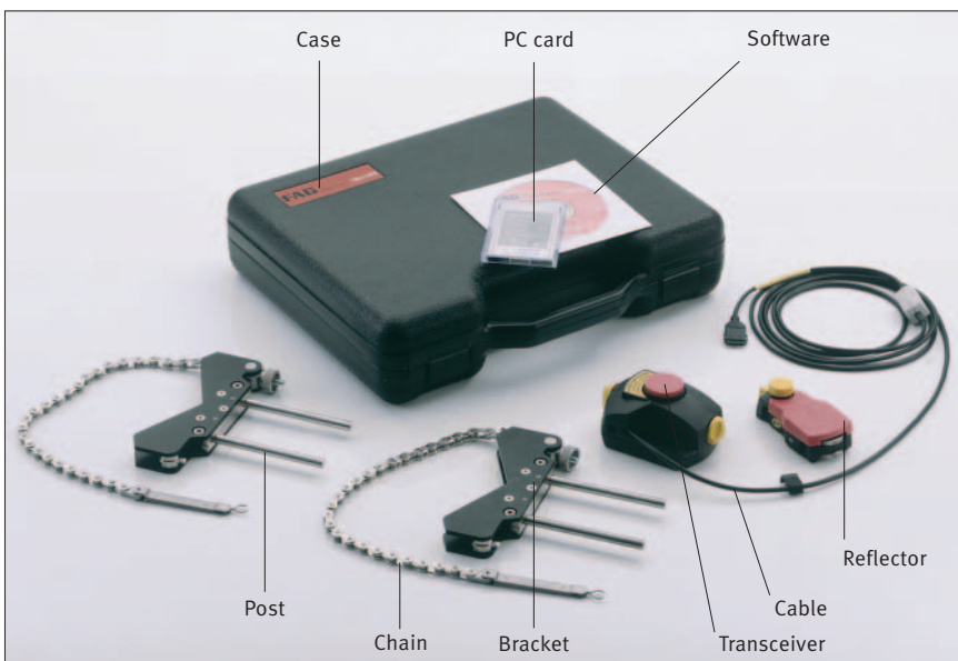
Scope of delivery of FAG Top-Laser INLINE
