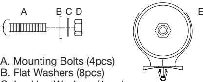
(Fig. 1) 90C - 92C - 95C Air Compressor Kit Installation Parts List:
