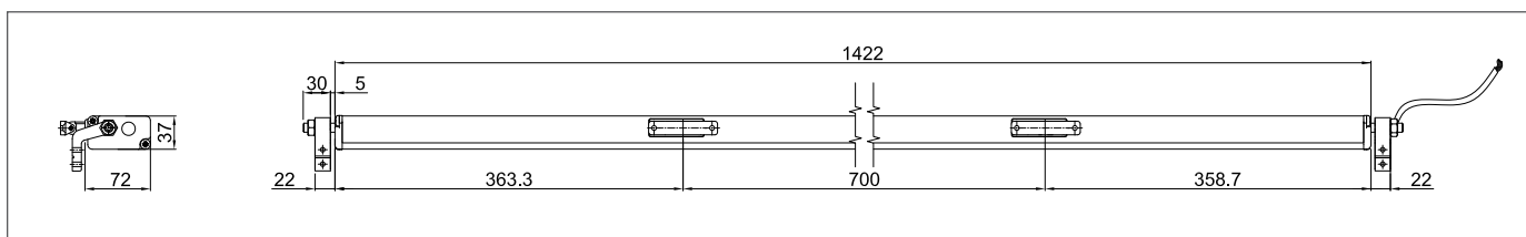
Twin Quasar dimensions
