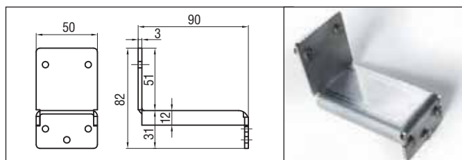
Stainless steel bottom hinged window bracket part No. 40858U
