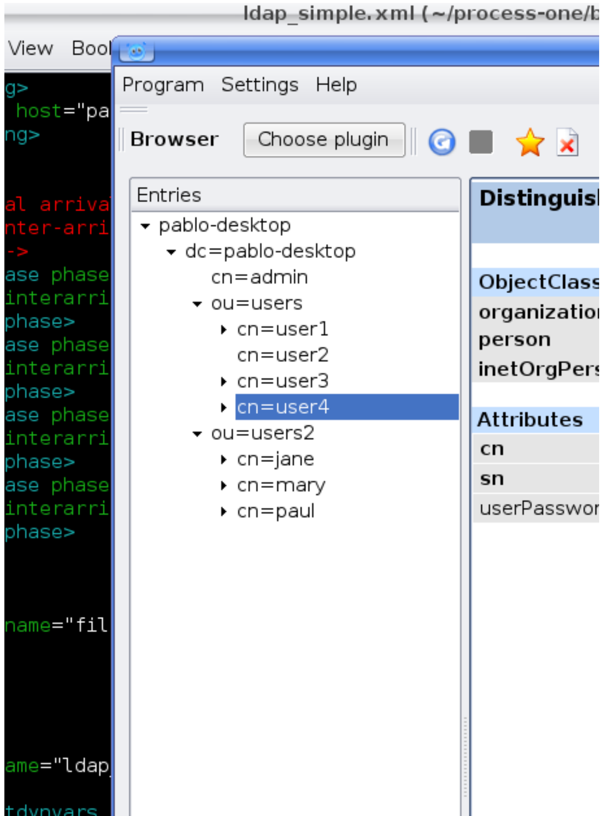
Figure 6.1: LDAP hierarchy
