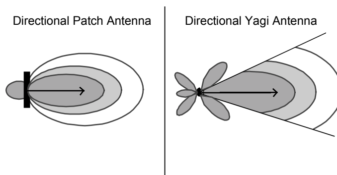
FIGURE 5.8 Coverage area of a semi-directional antenna
