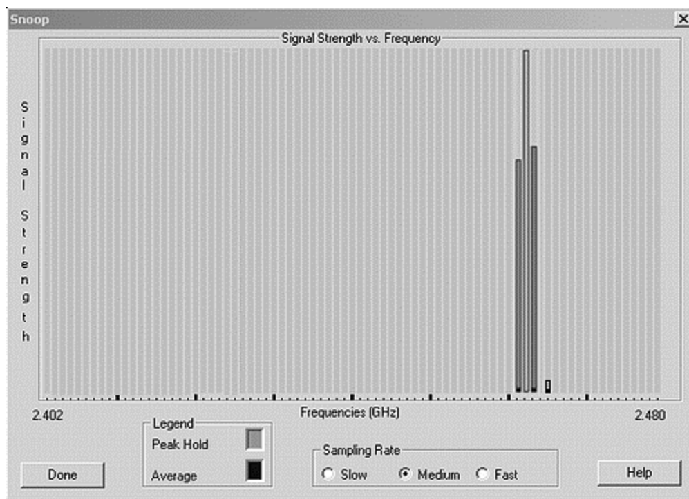
FIGURE 9.13 Screenshot of a spectrum analyzer showing narrowband interference
