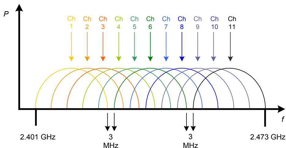
FIGURE 3.4 DSSS channel allocation and spectral relationship
