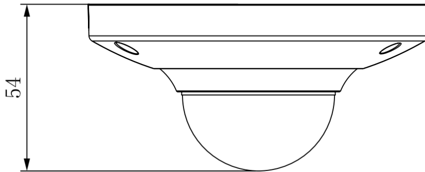
Figure 1-2 Dimension illustration 1
