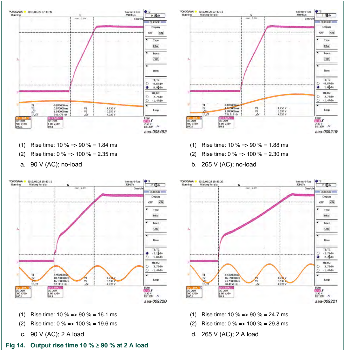
Figure 14 shows the rise time of the output from 10 % to 90 % at 90 V and 265 V with no-load and 2 A load.
