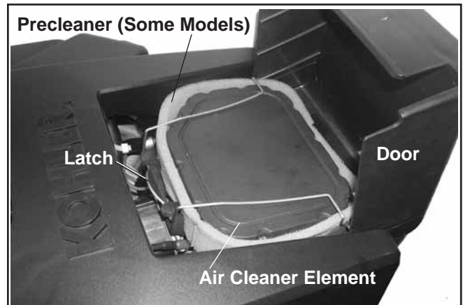
Figure 10. Courage Air Cleaner System.
