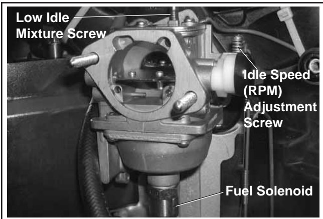
Figure 16. Carburetor Details.
