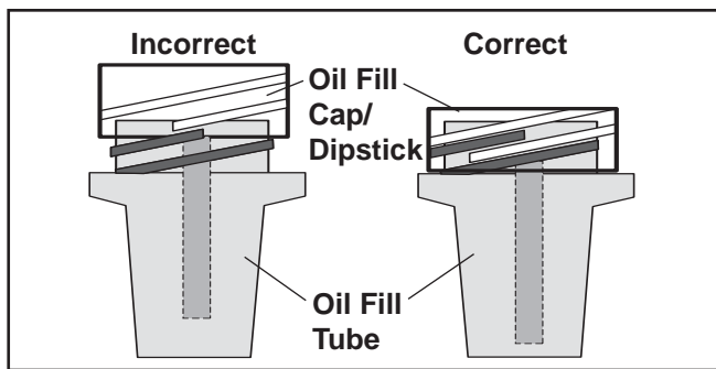
Figure 6. Thread-on Oil Fill Cap/Dipstick.
