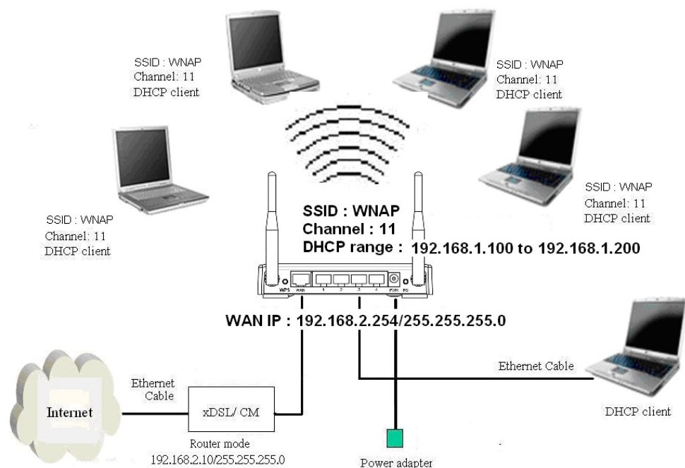
Figure 4 – Configuration Example Two – Fixed IP on the WAN
