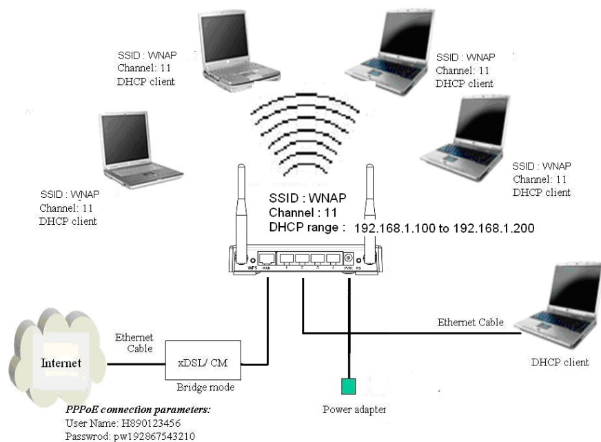
Figure 3 – Configuration Example One – PPPoE on the WAN
