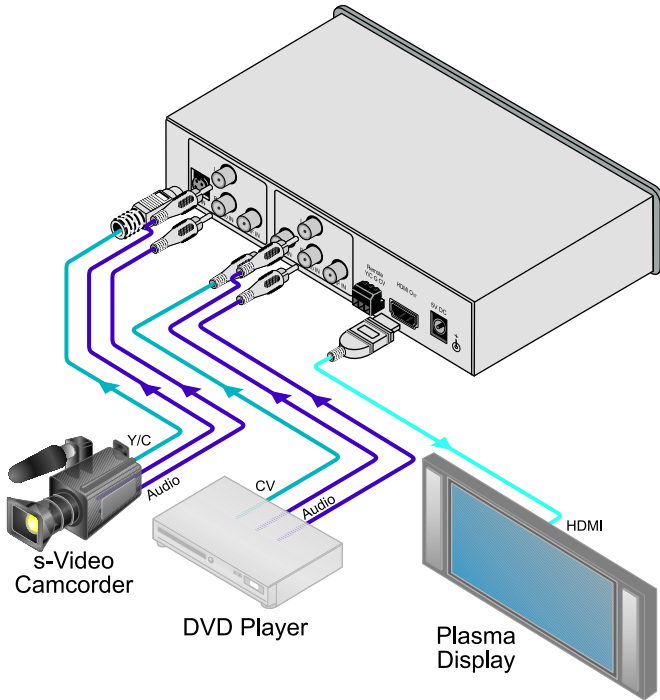
Figure 2: Connecting the VP-418xl Video to HDMI Scaler
