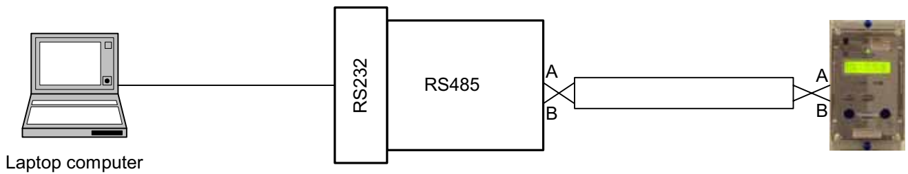
Figure 4.3-3 Communication to Argus Relay using RS485 – RS232 converter (Local Connection)
