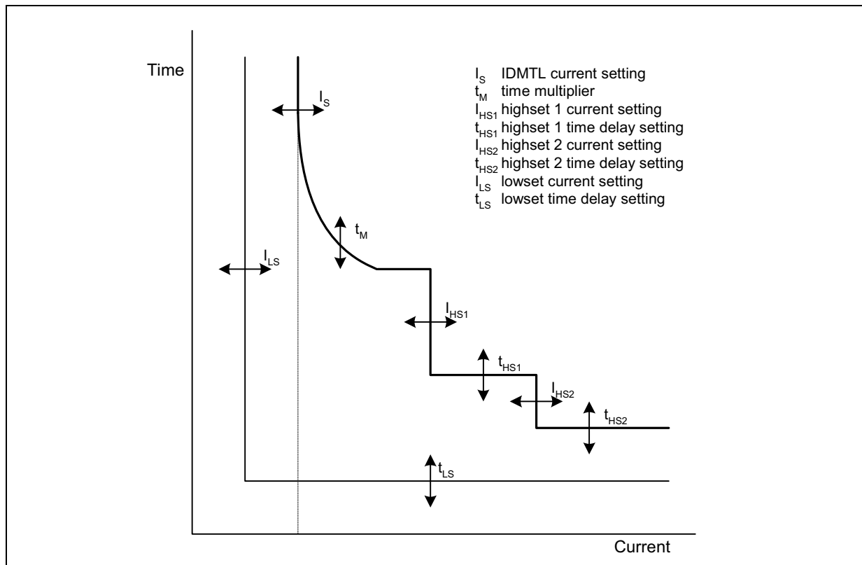
Figure 1-1 Overcurrent Characteristics
