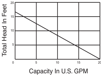
Low head pump curve
