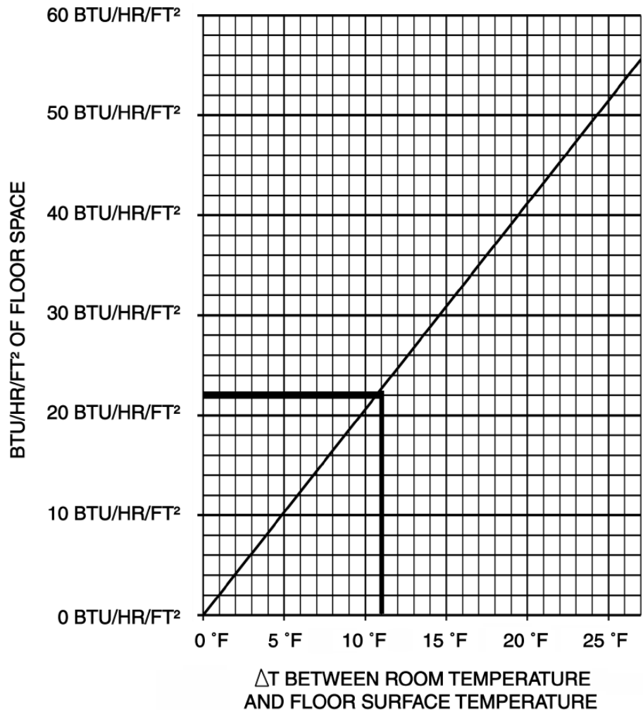
Floor Surface Temperature Chart
