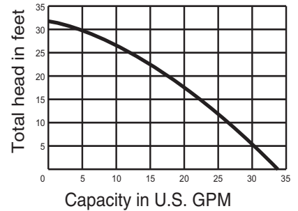
High head pump curve
