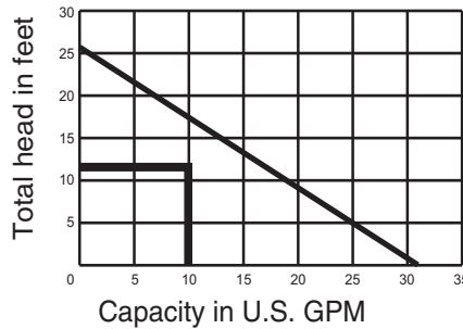
Medium head pump curve
