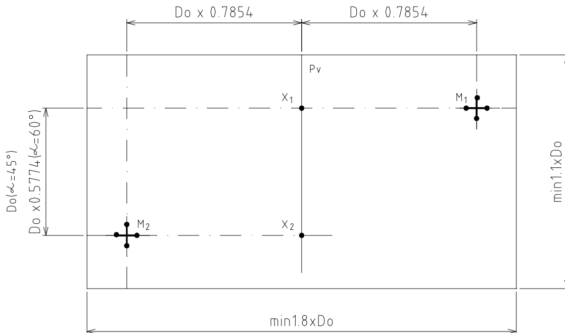
Fig. 22 Paper template
