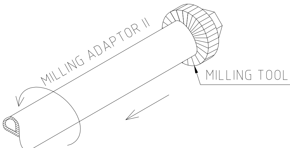
Fig. 26 Facing of the seating surface on the inaccessible welded-on piece
