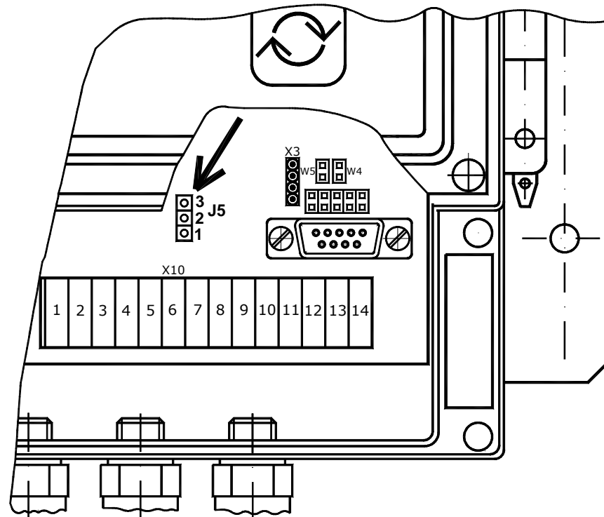
Fig. 38 Position of jumper J5
