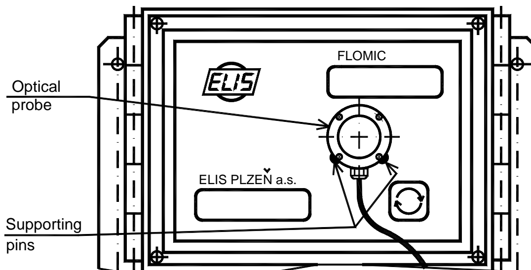
Obr.39 Working position of the optical probe
