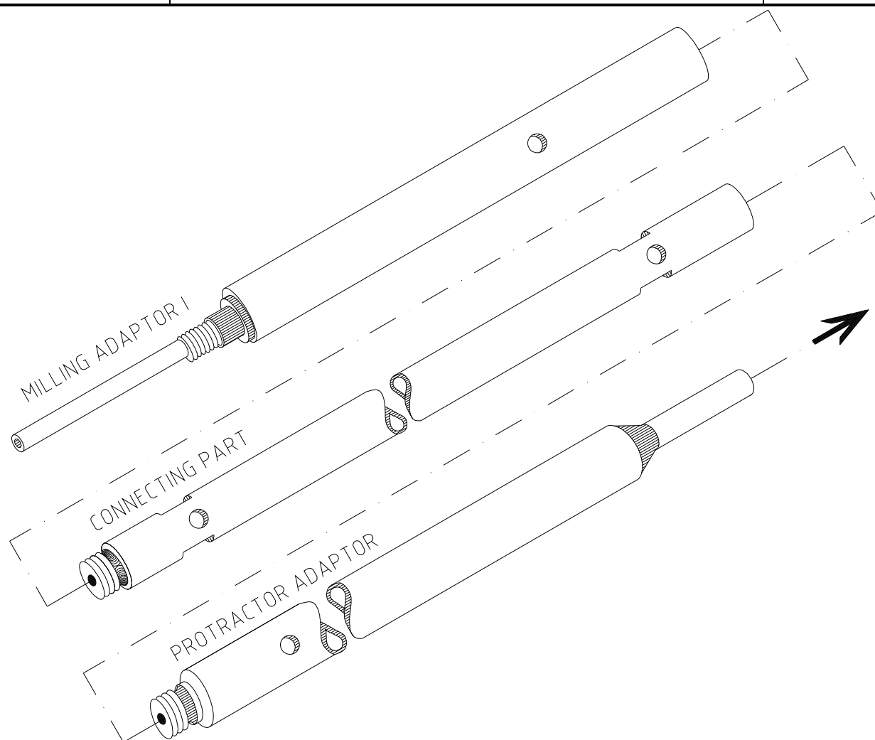
Fig. 24 Rectification pin assembly parts
