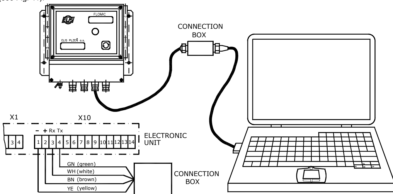
Fig. 41 Communication via RS 232 interface
