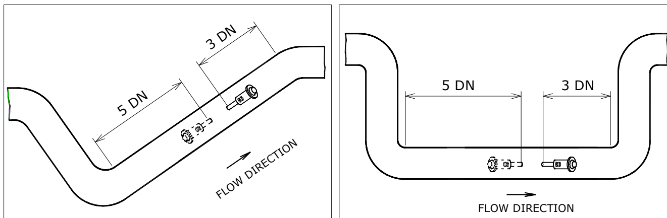
Fig. 16 Sensor placement in bottom pockets ensuring complete flooding at all times
