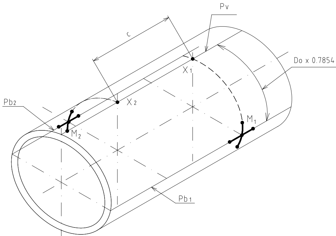
Fig. 21 Laying out of key installation points
