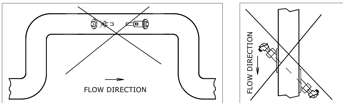
Fig. 18 Examples of incorrect sensor placement
