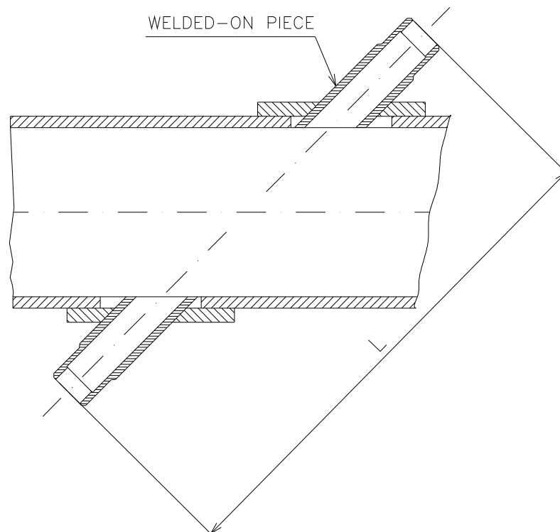
Fig. 28 Determination of distance L
