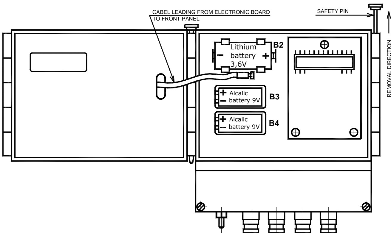
Fig. 43 Battery replacement
