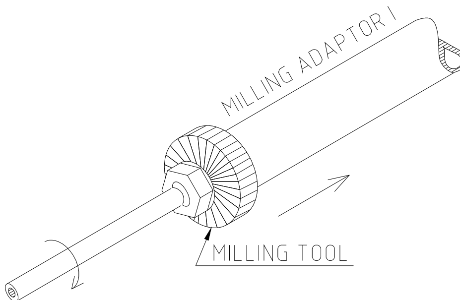
Fig. 25 Facing of the seating surfaces on the welded-on pieces
