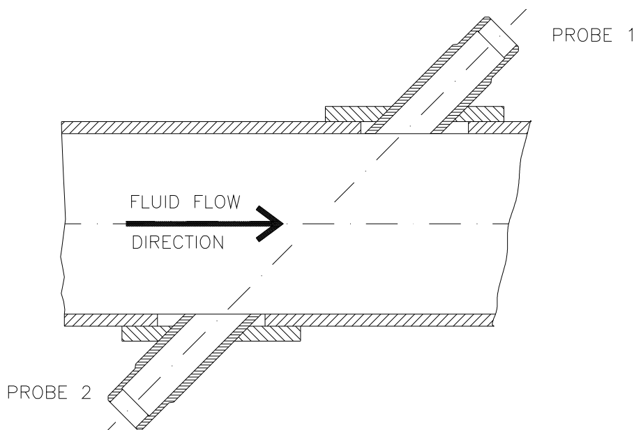
Fig. 30 Probe marking
