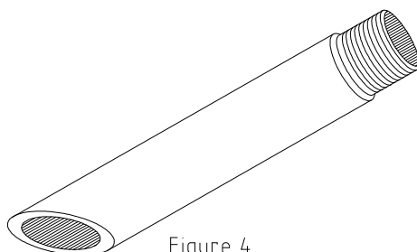
Figure 4 WELDED-ON PIECE
