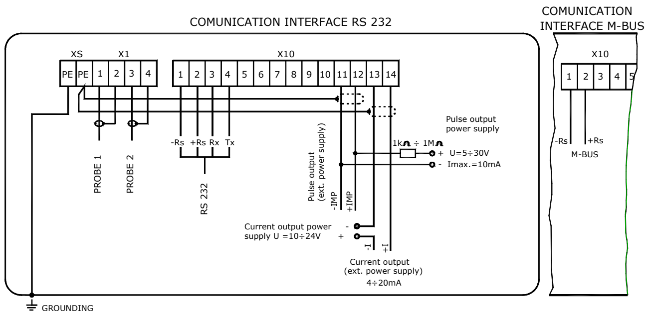
Fig. 29 Input and output signal connections of the UP 8.00 electronic unit
