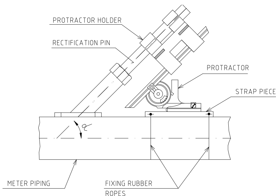
Fig. 27 Determination of the measuring ray angle
