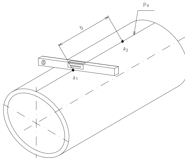
Fig. 20 Top surface line marking on meter piping.
