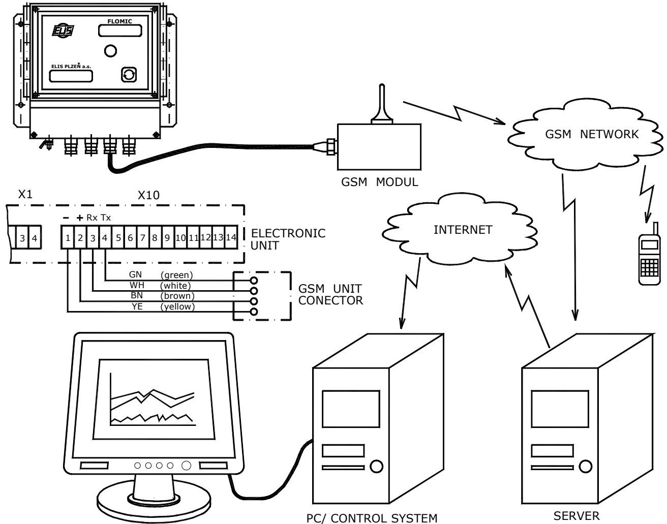
Fig. 42 Flow-meter data communication via a GSM port
