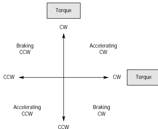
Fig. 2.18 Four-quadrant operation
