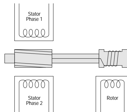
Fig. 4.22 Brushless resolver
