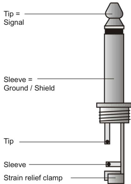
Unbalanced mono 1/4" jack plug
