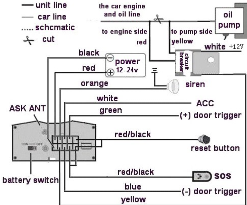
Wiring diagram
