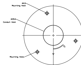
Drill template
