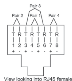
Figure 1-6. CAT5/5E/6 Straight Through UTP/STP Cable (8P8C)
