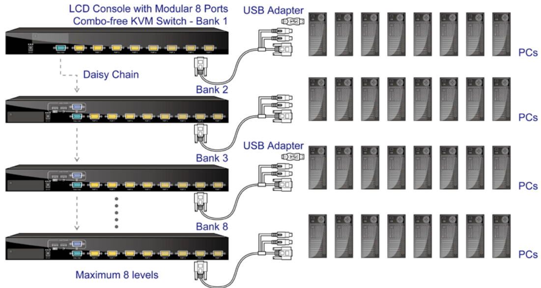
Figure 2-9. Daisy Chain Connection
