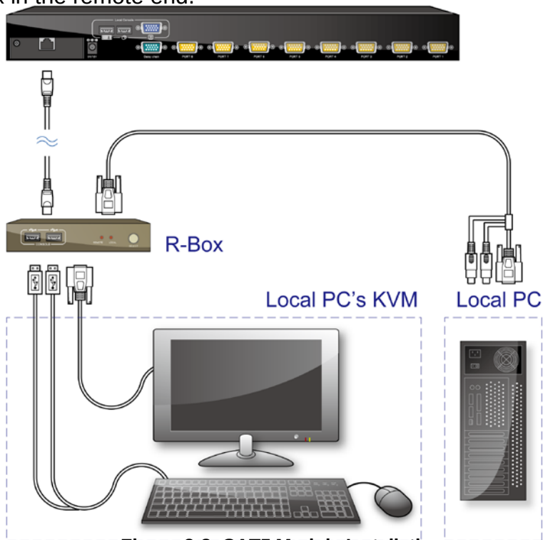
Figure 2-8. CAT5 Module Installation
