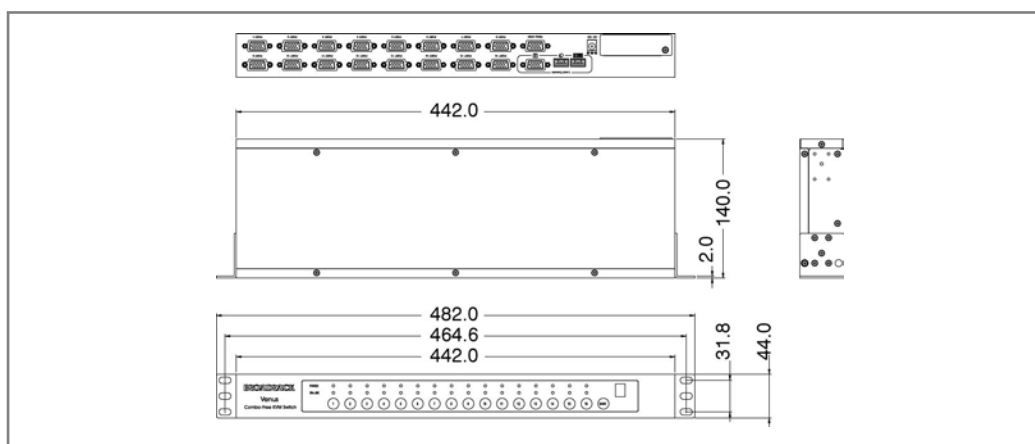
Figure 1-1. Venus 8 / 16 Series Dimensions
