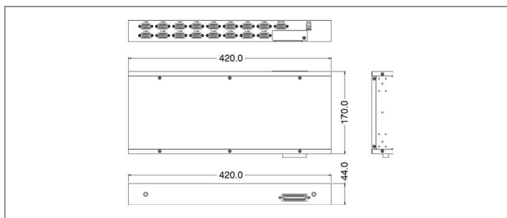
Figure 1-2. Venus 8D / 16D Series Dimensions
