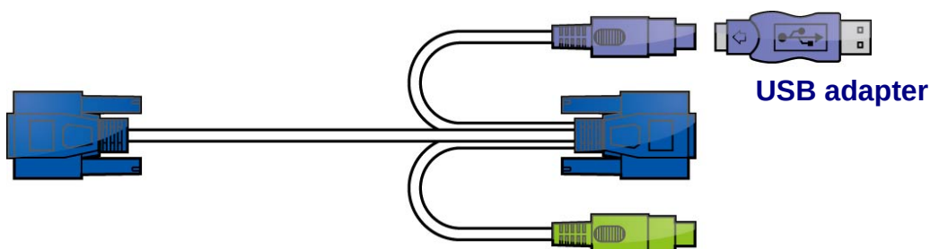
Figure 2-5. 3-in-1 HDDB-15 Cable with USB Adapter
