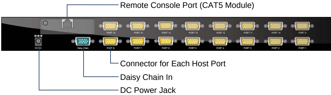
Figure 1-8. Rear Panel
