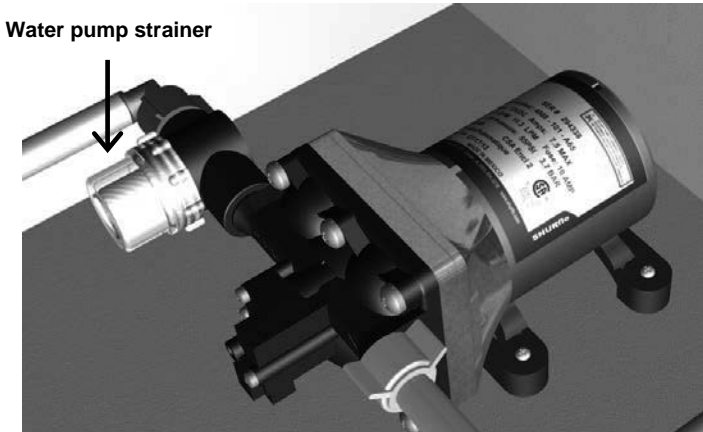
Fig. 8.1 Water pump
