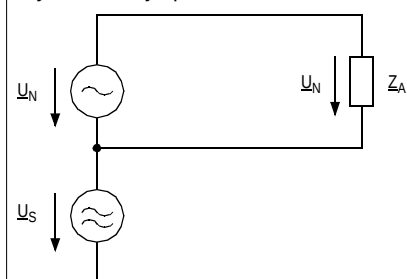
Common mode interference in an asymmetrically operated electrical circuit
