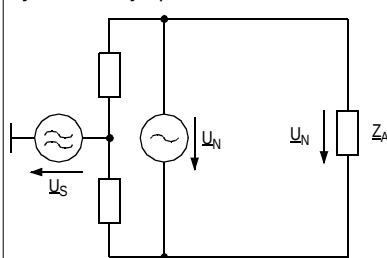
Common mode interference in a symmetrically operated electrical circuit
