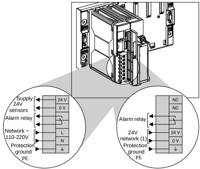
Alternating current supply TSX PSY 2600/5500/8500
