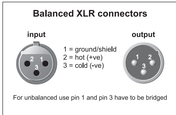
Fig. 4.2: XLR connections
