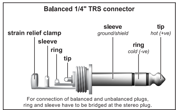
Fig. 4.4: 1/4" TRS connector
