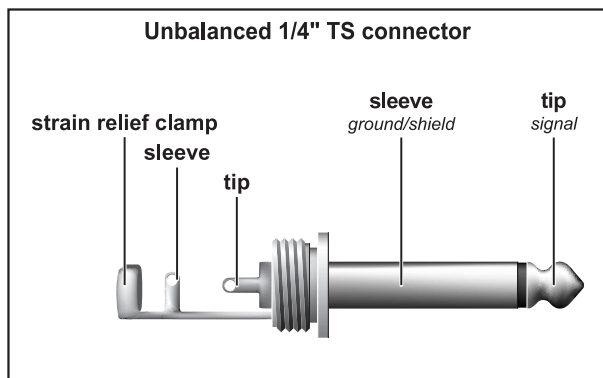
Fig. 4.3: 1/4" TS connector
