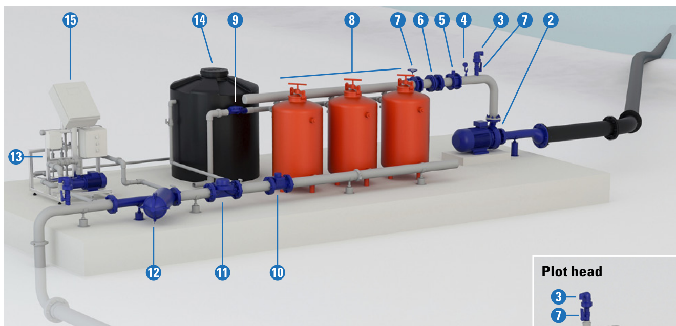
System head
