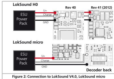
Figure 2: Connection to LokSound V4.0, LokSound micro
