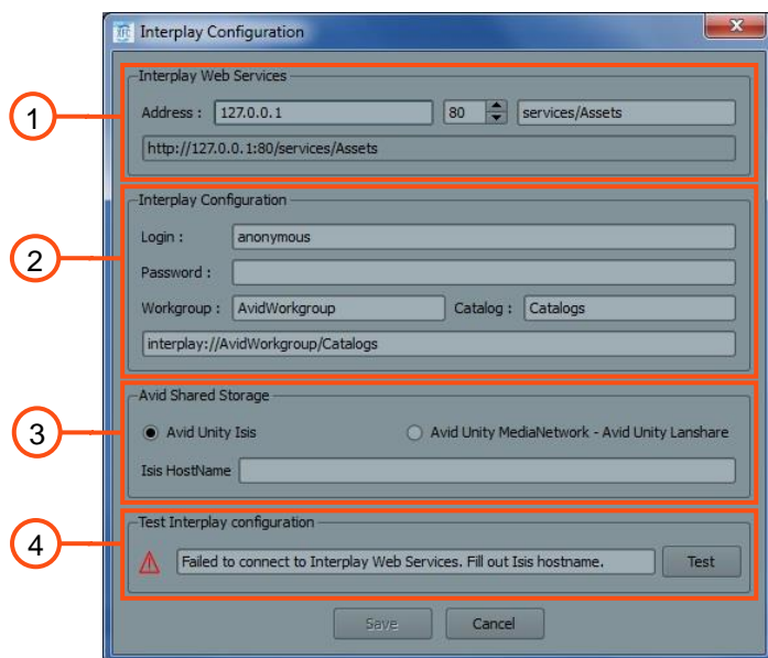
Figure 38: Interplay configuration
