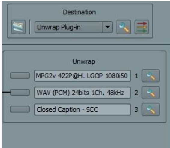
Figure 19: Unwrap plug-in
