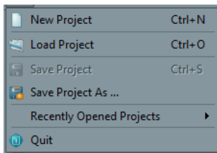
Figure 6: File menu
