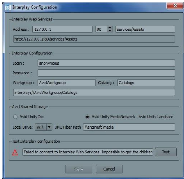
Figure 39: Lanshare settings
