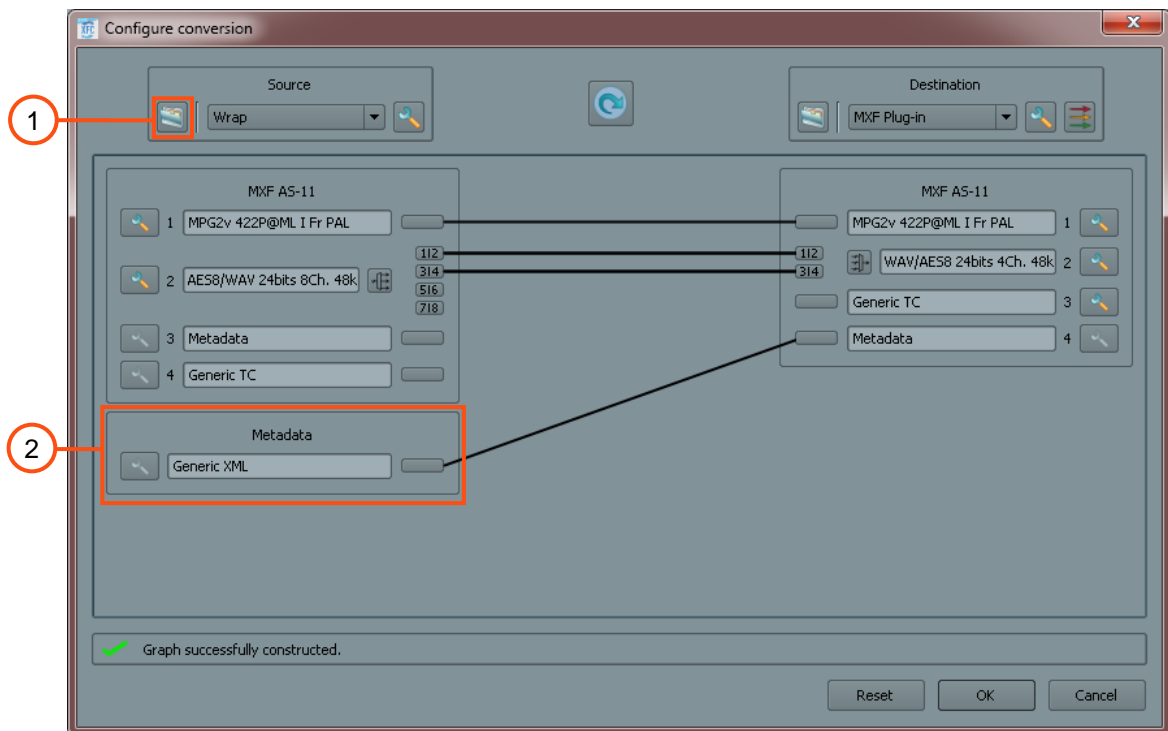
Figure 16: How to define AS-11 Metadata
