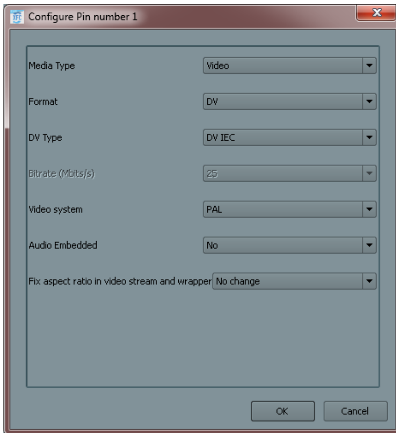
Figure 21: Force Aspect Ratio in DV stream
