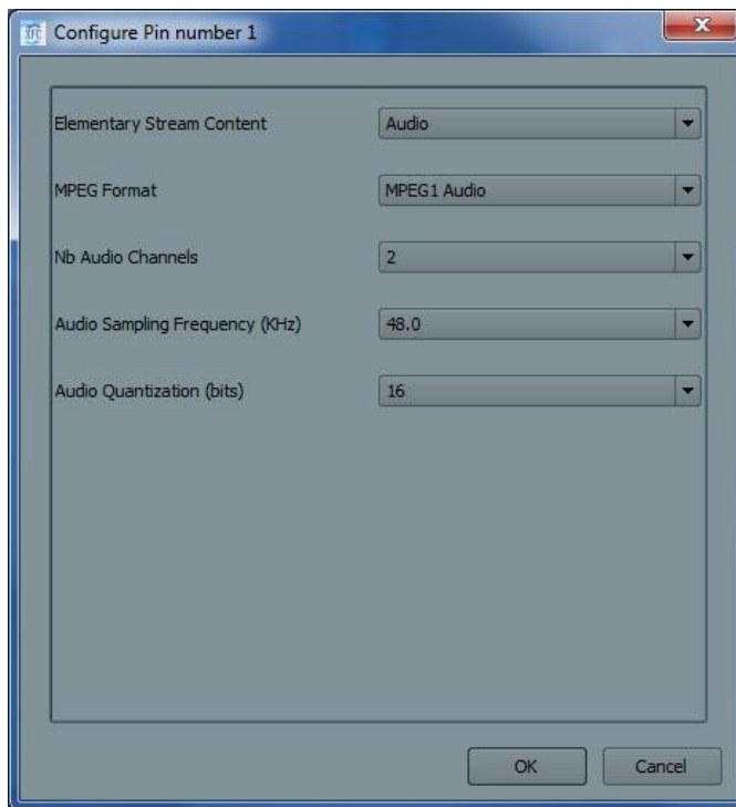
Figure 26: MPEG-1, MPEG-2 and AAC audio elementary stream settings
