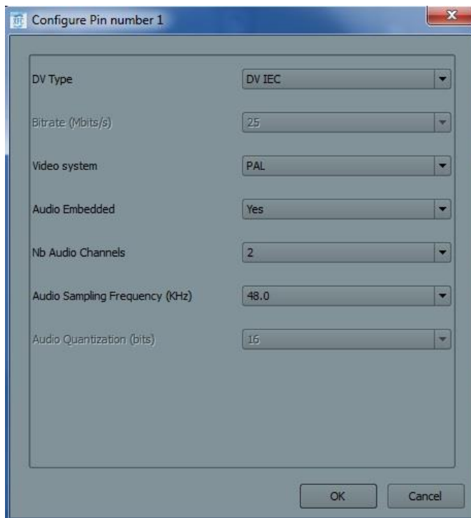
Figure 20: DV stream settings
