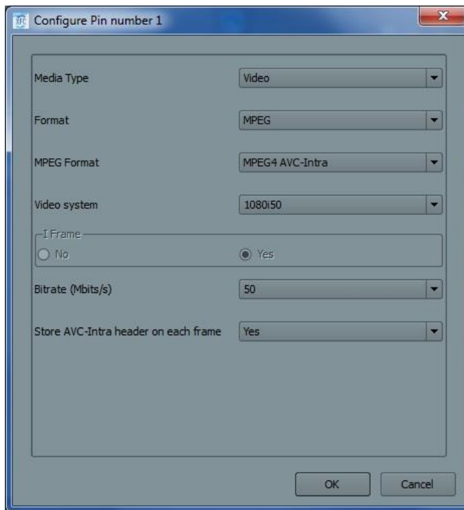
Figure 24: AVC-Intra elementary stream settings
