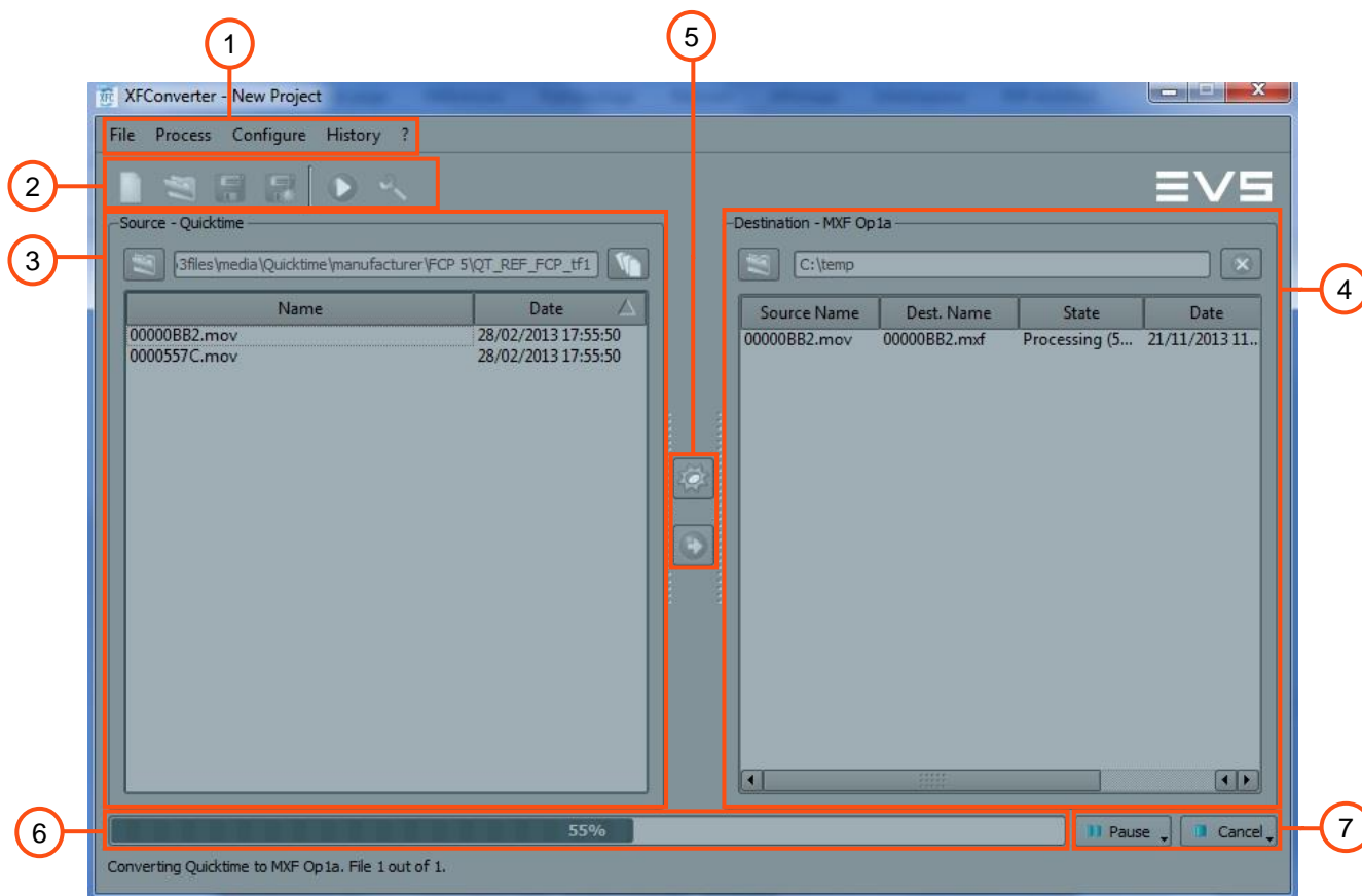
Figure 3: OpenCube XFConverter main window
