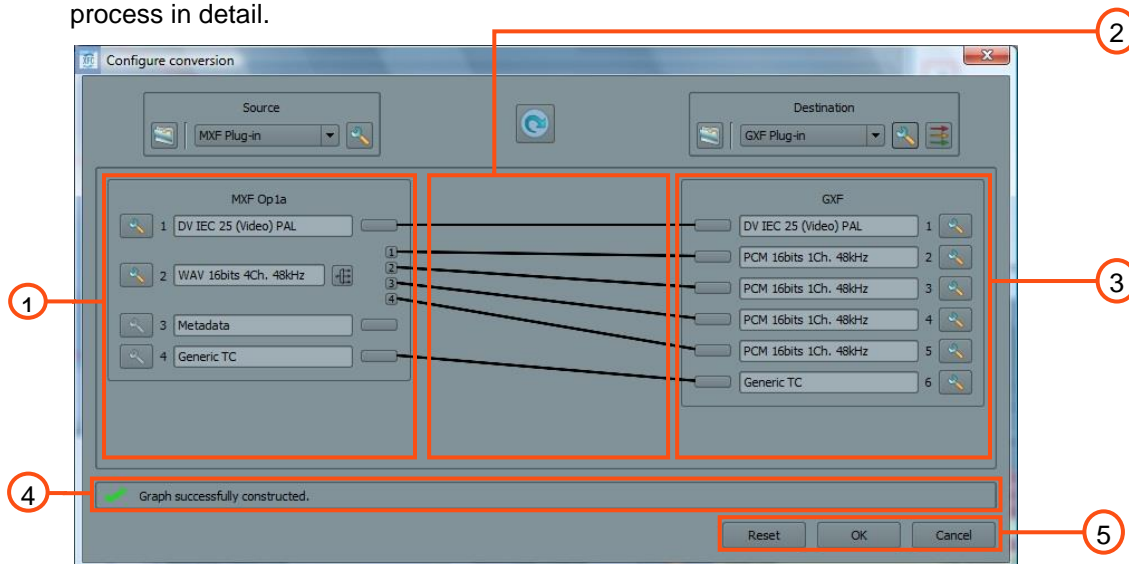
Figure 7: Configure conversion window
