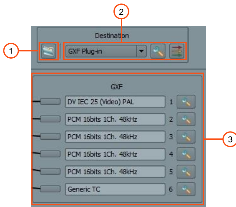
Figure 9: Configure conversion window - Destination part
