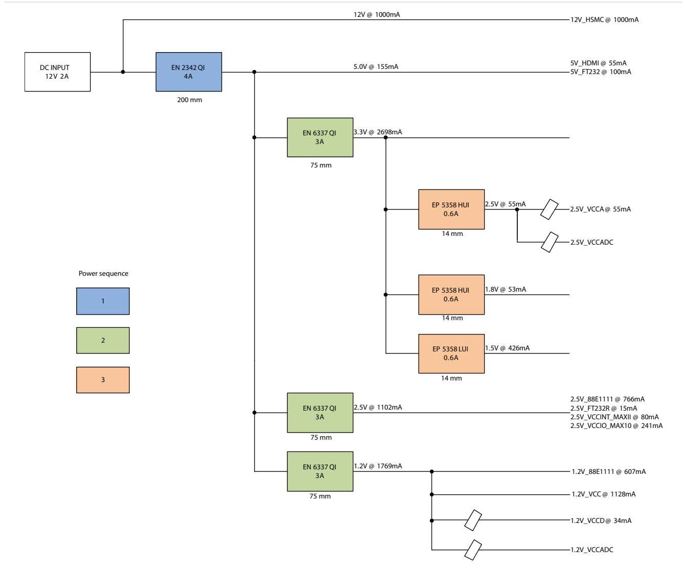
Figure 4-4: Power Distribution System
