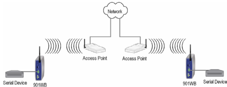
Figure 5. Serial Tunneling via Infrastructure
