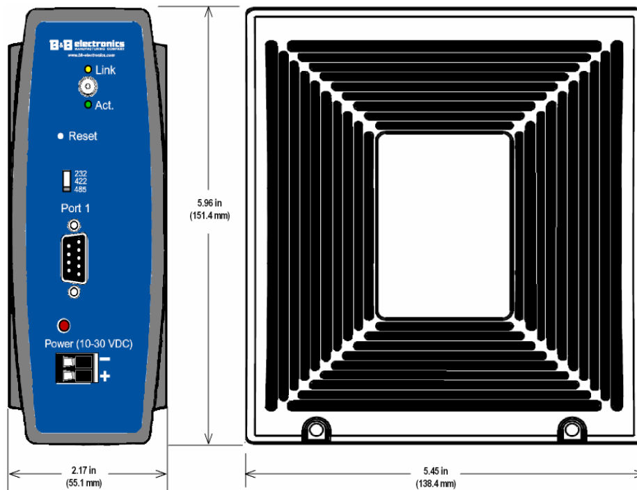
Figure 17. Dimensional Diagram of the ESR901WB
