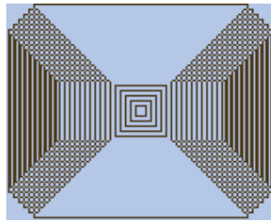
Figure 12.36.: Mosaique
