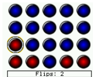
Figure 12.9.: Flipit
