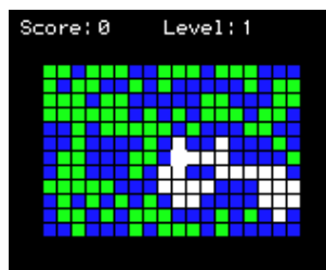
Figure 12.5.: Clix
