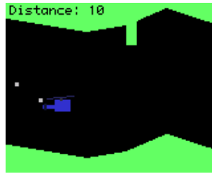
Figure 12.6.: Chopper
