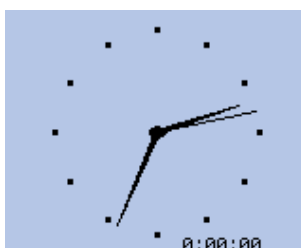
Figure 12.51.: Clock
