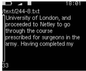
Figure 12.44.: Text Viewer
