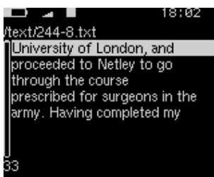
Figure 12.46.: A bookmark
