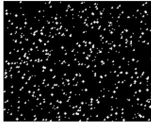
Figure 12.41.: Starfield
