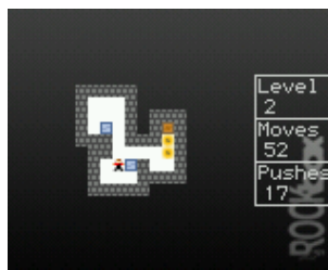
Figure 12.24.: Sokoban
