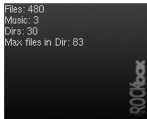
Figure 12.54.: The stats-plugin
