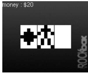
Figure 12.12.: Jackpot
