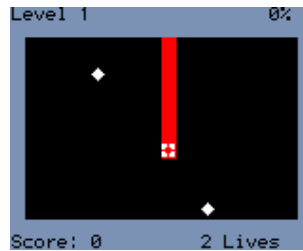
Figure 12.30.: Xbox
