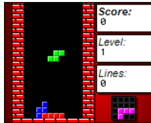
Figure 12.20.: Rockblox
