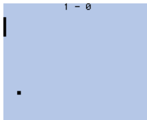
Figure 12.18.: Pong
