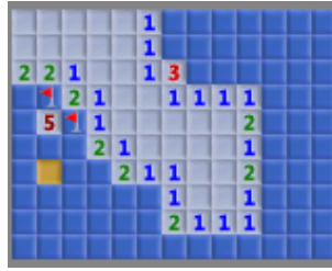
Figure 12.15.: Minesweeper plugin
