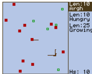
Figure 12.29.: Wormlet game
