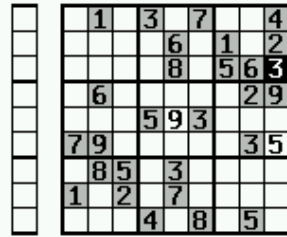
Figure 12.28.: Sudoku
