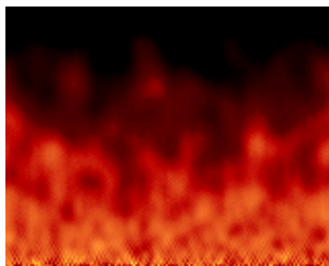
Figure 12.34.: Fire
