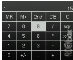
Figure 12.48.: Calculator
