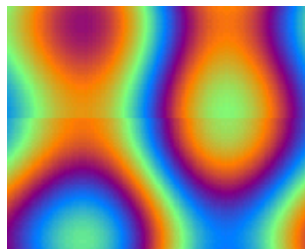
Figure 12.39.: Plasma
