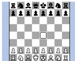
Figure 12.4.: Chessbox
