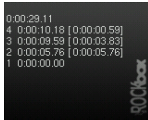
Figure 12.55.: Stopwatch
