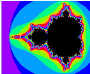
Figure 12.35.: Fractals: Mandelbrot set
