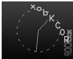
Figure 12.31.: Bounce
