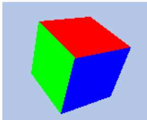
Figure 12.32.: Cube
