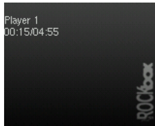
Figure 12.50.: Chess Clock
