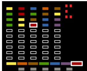
Figure 12.7.: Codebuster
