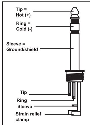
Balanced/stereo 1/4" jack plugs
