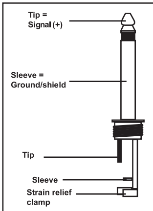
Unbalanced mono 1/4" jack plugs
