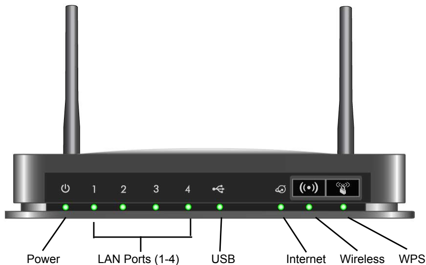
Figure 1 Front panel
