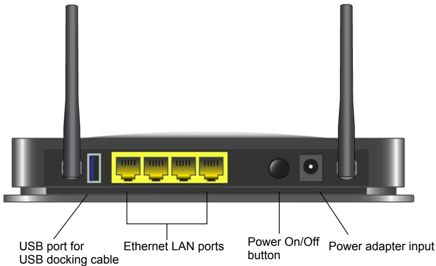
Figure 2 Back panel
