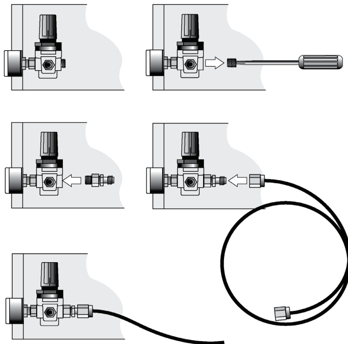
Figure 3 Gas Tube Connection from Pressure Regulator to SPME Fiber Conditioning Station
