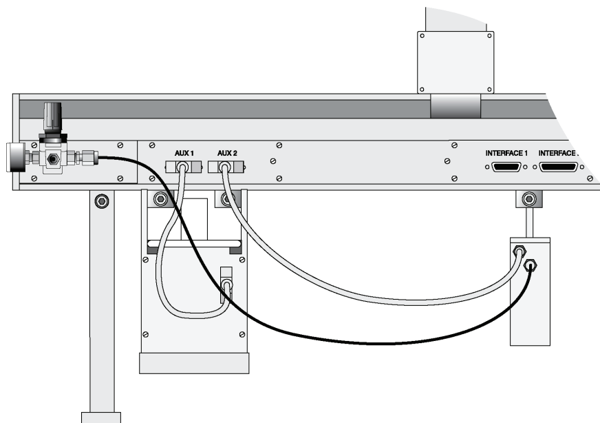
Figure 2 SPME Fiber Conditioning Station, Electrical and Gas Connections
