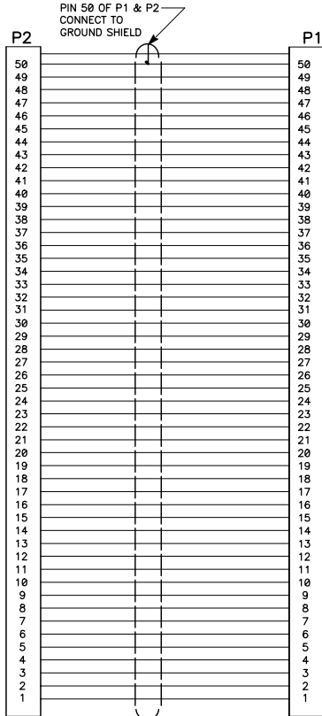
MODEL 5025-551-x SCHEMATIC MODEL 5025-551-x SIGNAL CABLE, SHIELDED 4501-463A
