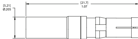
Receiver Contact Part # 610 104 133
