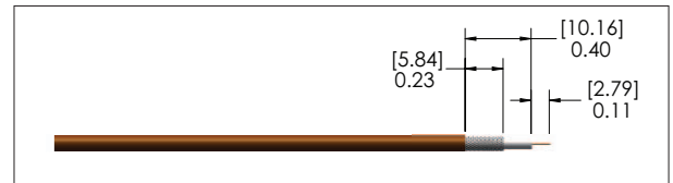
Figure A. Strip lengths.
