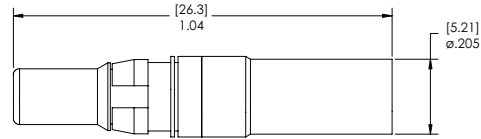
ITA Contact Part # 610 102 132
