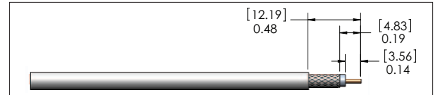
Figure A. Strip lengths.
