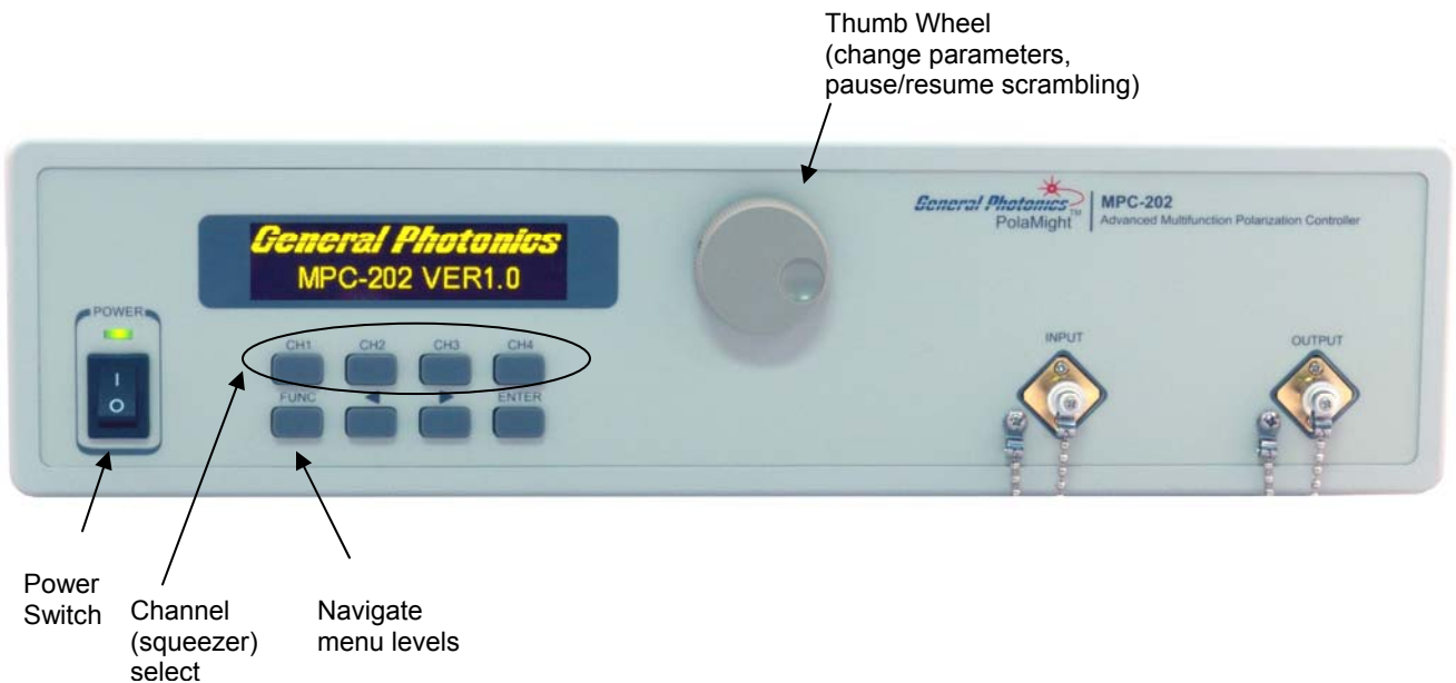
Figure 4 MPC-202 front panel
