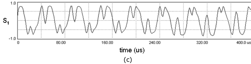
Figure 14 10 second SOP capture of tornado scrambling: (a) randomly rotating spin axis at 20 revolutions per second, (b) fixed rotating spin axis at 100 rev/s. (c) Tornado scrambling rate of 40,000 revolutions/s confirmed by measurement of one of the three Stokes parameters vs time, measured using the oscilloscope mode of a General Photonics polarimeter. The measured periodicity is 25 \mu s per revolution, or 40,000 rev/s.
