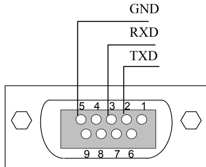
Figure 27 RS-232 connector pin assignment on MPC-202 rear panel.
