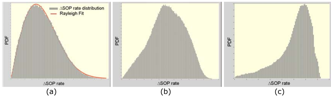
Figure 15 SOP variation rate distributions of (a) Rayleigh, (b) Triangle, and (c) Tornado scrambling.
