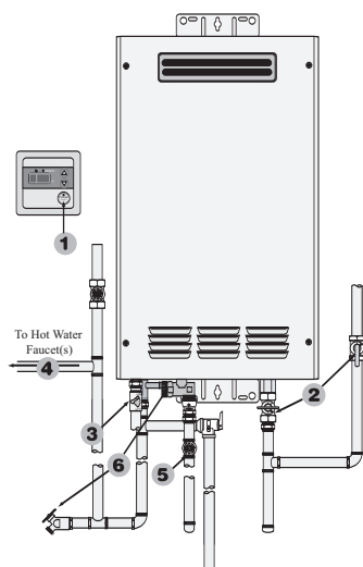
Draining the water heater
