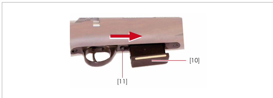
Fig.12 Sliding the magazine holder forwards
