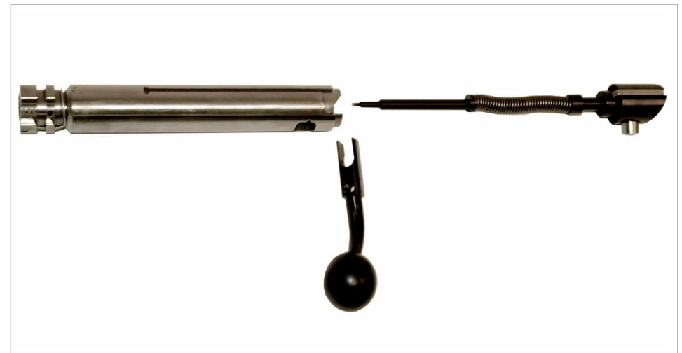
Fig.26 Dismantled bolt
