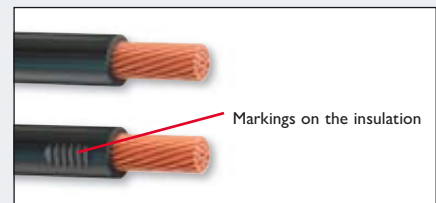
Correctly stripped cable in accordance with DIN IEC 60352
